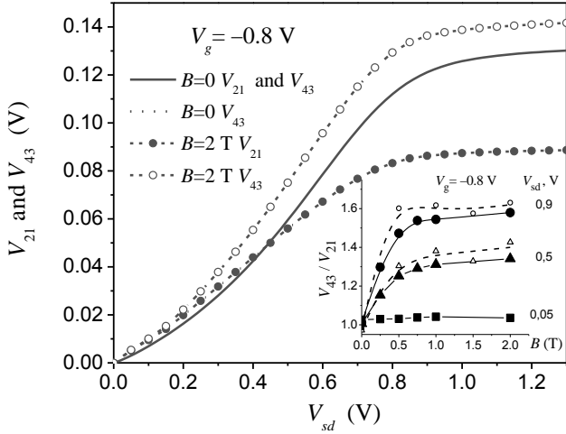
FIG. 8. Measured side voltages V_{21} and V_{43} as functions of the source-drain voltage V_{sd} . Solid line - at B=0 . Open and full circles - at B=2 T. Inset: Full symbols and solid lines: measured ratio V_{43}/V_{21} as a function of magnetic field for several values of V_{sd} . Open symbols and dashed lines: calculation on the basis of results for the linear regime in Fig. 5, using Eq. (10).
