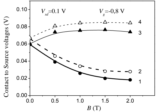
Fig. 5. Voltages measured between side contacts 1–4 and the source as functions of magnetic field B . Note the saturation at B > 1 T.
