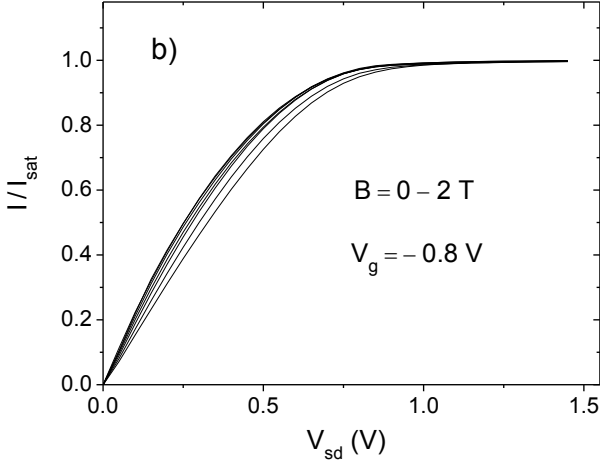
FIG. 6: (a) I vs V_{sd} dependencies for several values of magnetic field at V_g = -0.8 V. (b) I/I_{sat} vs V_{sd} curves for several values of magnetic field and fixed V_g = -0.8 V.
