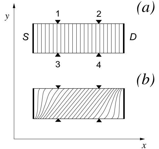
FIG. 1: Schematics of the equipotential lines for a Hall bar with source (S) and drain (D) contacts: (a)- at zero magnetic field, (b) - in the presence of magnetic field. Side contacts for measuring Hall and longitudinal voltages are shown. In our samples, the contacts 1, 3 and 2, 4 are situated symmetrically with respect to the middle of the sample.
