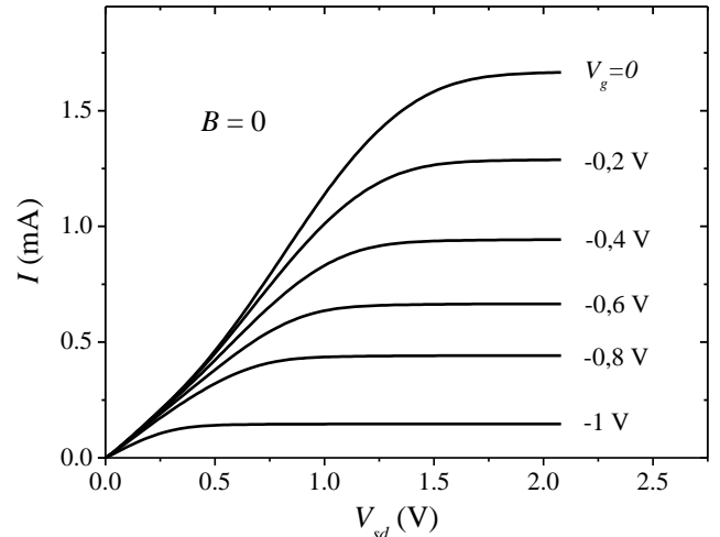
FIG. 3. Measured I - V dependencies at B = 0 for different values of the gate voltage V_g = V_{th} + V_s .
