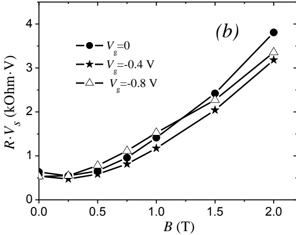
Fig. 4. (a) Magnetoresistance R(B) in the linear regime ( V_{sd} = 0.1 V) for several values of V_g . Inset: R(B)/R(0) and R_{21}(B)/R_{21}(0) at V_g = -0.8 V, V_{sd} = 0.1 V. (b) Product R \cdot V_s , as a function of B for the same values of V_g .
