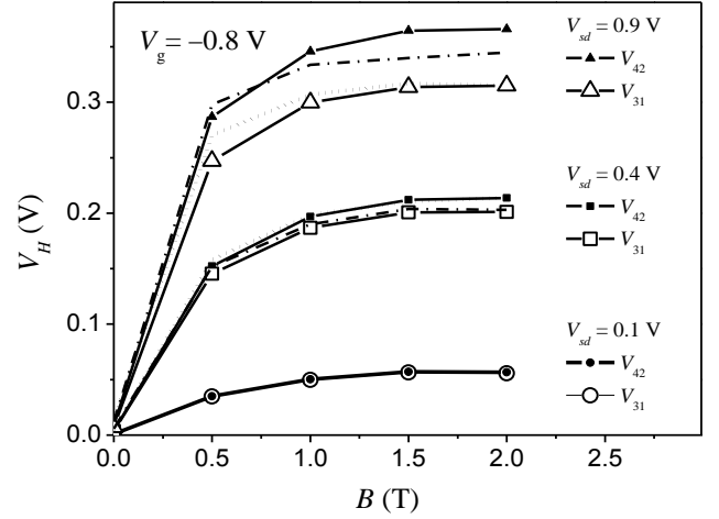
FIG. 7: The Hall voltage V_H as a function of magnetic field measured between two pairs of contacts, 3, 1 and 4, 2 in the linear regime ( V_{sd} = 0.1 V), weakly nonlinear regime ( V_{sd} = 0.4 V) and strongly nonlinear regime ( V_{sd} = 0.9 V). Dashed lines: calculation on the basis of results for the linear regime in Fig. 5, using Eq. (10).
