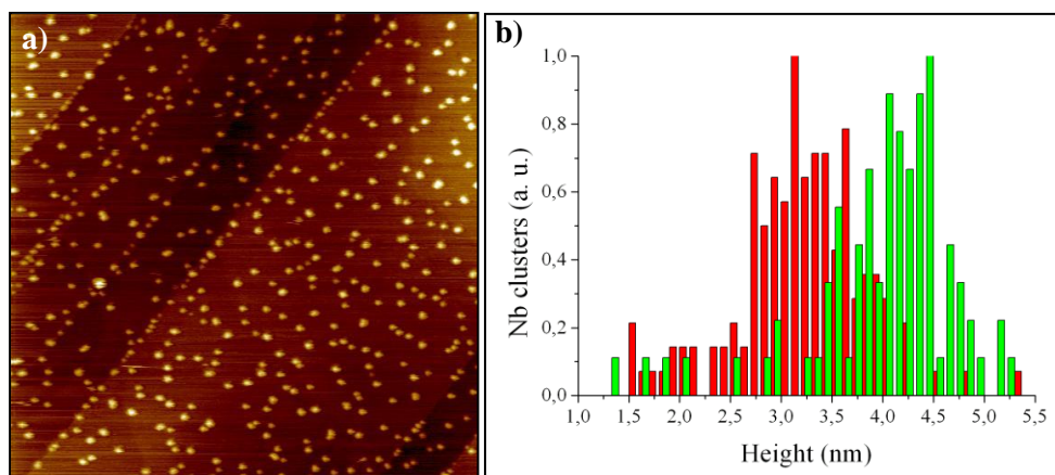
FIG. 1: (a) AFM image of Au 2000 clusters soft-landed on Ar + sputtered graphite after silver evaporation (3μm x 3μm). (b) Height distribution of the clusters before (red) and after (green, as (a)) one 1/100 silver monolayer evaporation.
