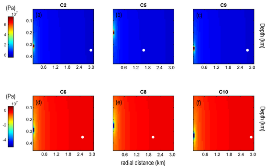
Fig. 6. Excess pore pressure distribution in axisymmetric coordinate system calculated using poroelastic models. (a)-(c) are results of three injection wells, C2, C5 and C9 respectively, and (d)-(f) are their corresponding pumping wells, C6, C8 and C10, respectively. The white dot marks the hypocenter location from Yi et al., 2019. Note the maximum and minimum excess pore pressure at each plot is the injection/pumping spot in the salt mine formation. The vertical depths of the injection/pumping spots are from 2644 m to 3153 m, and the hypocenter of the Changning earthquake is at 3000 m.
