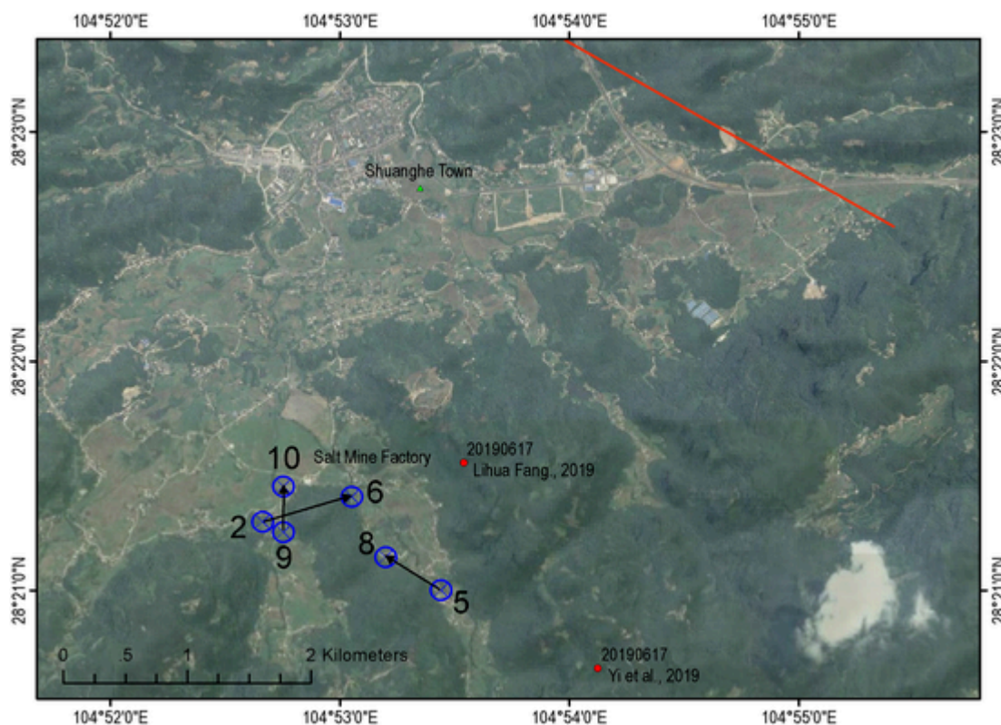
Fig. 5. Ground locations of salt mine wells and inferred hypocenters of Changning earthquake. The blue circles with cross inside show the salt well locations, and the black arrows denote the fluid flow directions at salt formation. The wells are named C2, C6, C9, C10, C5, and C8 with a number labeled at each well, and the salt mine factory is located near well C6. The red points show the epicenters from different groups. The red line indicates the fault top ground projection near the Shuanghe town. (For interpretation of the references to colour in this figure legend, the reader is referred to the web version of this article.)
