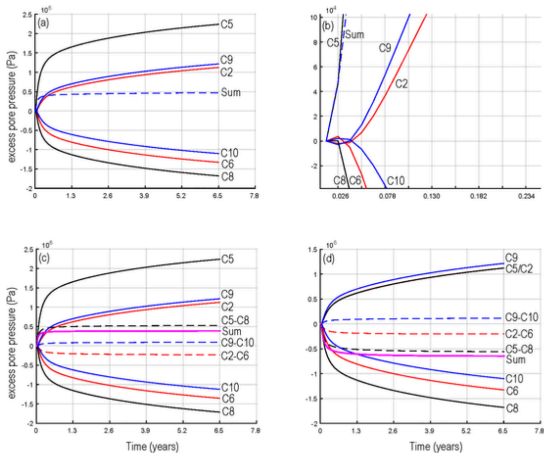
Fig. 7. Temporal behaviors of excess pore pressure at the hypocenter driven by injection and pumping operations. (a) Each solid curve represents the excess pore pressure evolution with time of individual well. The dashed line denotes the linear combination of the excess pore pressures from all of the 6 wells. (b) Zoomed in plot in (a) for showing the Noodberge effect at the early stage of mining operations. (c) Same as in (a), but with 0.5 \times 10^4 \text{ m}^3/\text{month} water loss at each well. The dashed lines show the excess pore pressure differences between each pair of injection and pumping wells. The magenta point-line denotes the linear combination of the excess pore pressures from all of the 6 wells. (d) Same as in (c), but well C5 is moved away from the hypocenter of the Changning earthquake. Note C5 and C2 curves overlap in this plot. (For interpretation of the references to colour in this figure legend, the reader is referred to the web version of this article.)
