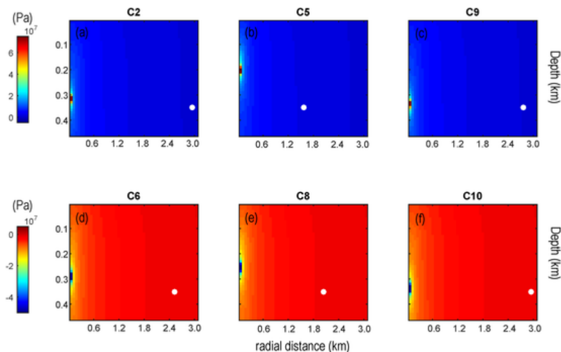
Fig. 6. Excess pore pressure distribution in axisymmetric coordinator system calculated using poroelastic models. (a)-(c) are results of three injection wells, C2, C5 and C9 respectively, and (d)-(f) are their corresponding pumping wells, C6, C8 and C10, respectively. The white dot marks the hypocenter location from Yi et al., 2019. Note the maximum and minimum excess pore pressure at each plot is the injection/pumping spot in the salt mine formation. The vertical depths of the injection/pumping spots are from 2644 m to 3153 m, and the hypocenter of the Changning earthquake is at 3000 m.
