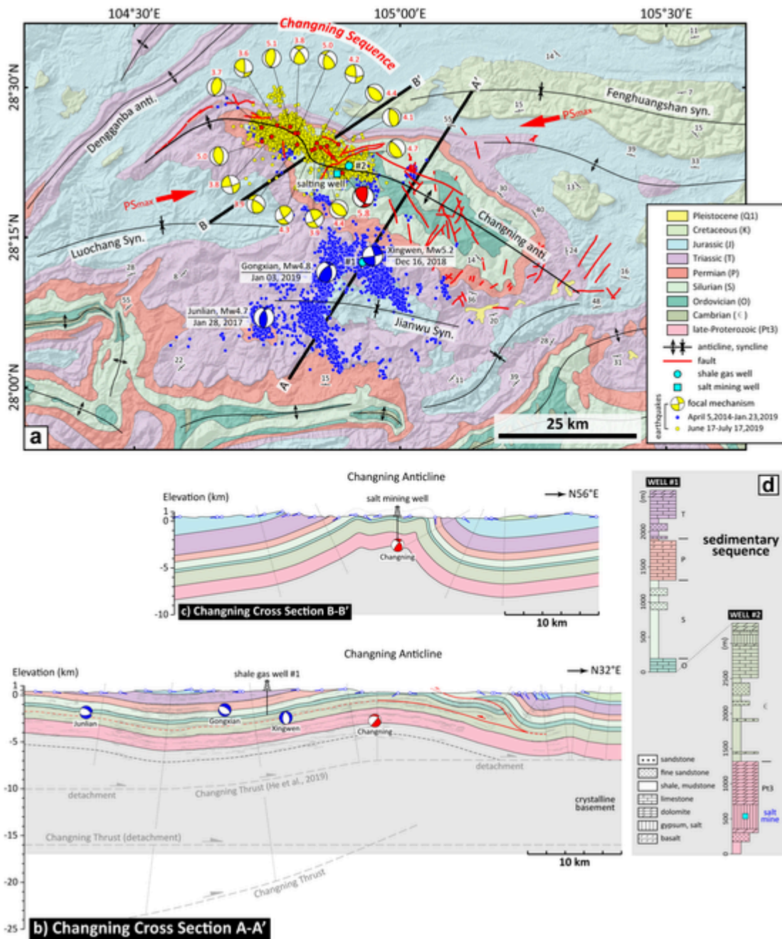
Fig. 2. (a) Geologic map of Changning anticline and its correlation with seismicity (Lei et al., 2019b). Orientation of the maximum compressional principal stress ( PS_{max} ) is from Jiang et al. (2020) and Lei et al. (2019b). The focal mechanisms of the 2019 Changning earthquake sequence are from Yi et al., (2019). (b) Geologic cross-section A-A' of the Changning fold interpreted from a seismic reflection profile of this study (see Fig. 2a for the location). Geometry of the Changning thrust beneath the Changning fold is speculative. (c) Geologic cross-section B-B' of the Changning fold based on surface mapping data (see Fig. 2a for the location). (d) The sedimentary sequence at Well #1 and #2 (after He et al., 2019). See Fig. 2a for the wells' locations.
