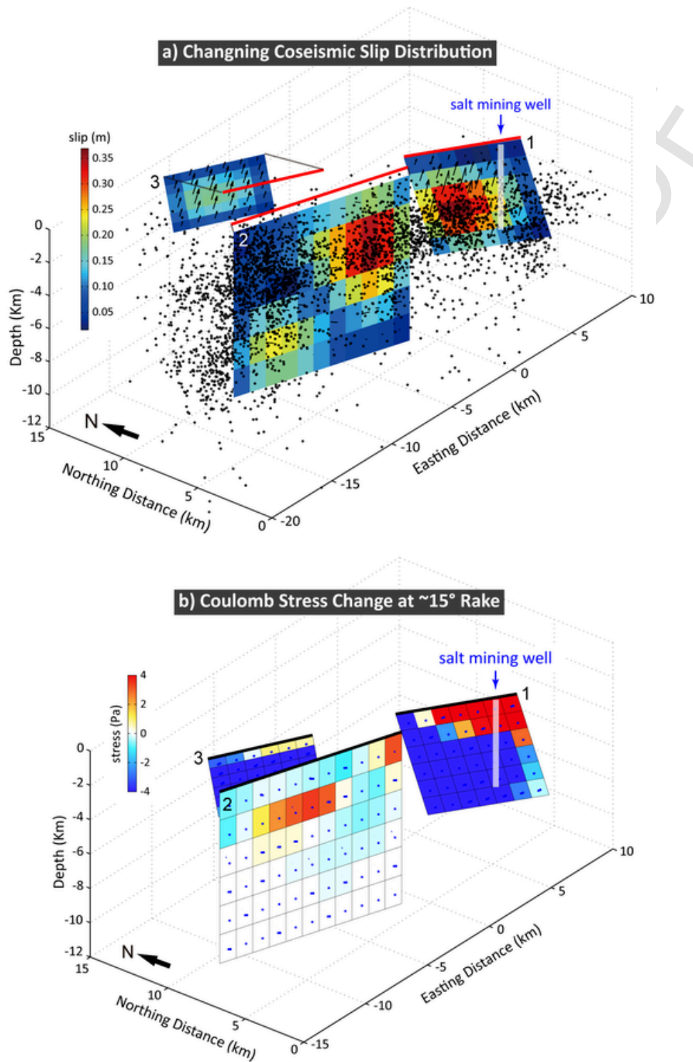
Fig. 4. (a) Fault geometry and slip distribution inverted from InSAR data. (b) Coulomb stress changes at \sim 15^\circ rake on the segment 2. The source fault is the segment 1 with its thrust-dominated slip distribution, and segment 2 and 3 are the receiver faults.
