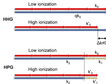
Fig. 5. Schematic comparison of the HHG and HPG phase matching and blue shift with the presence of low and high ionization. The high electronic density creates a phase mismatch \Delta k \neq 0 in case of HHG. In the case of HPG, the change of the fundamental k_0 is compensated by the change of k_1 so \Delta k = 0 is valid even under high ionization and the RSS (wave number k_2 ) are phase-matched and keep their spectral frequency.
