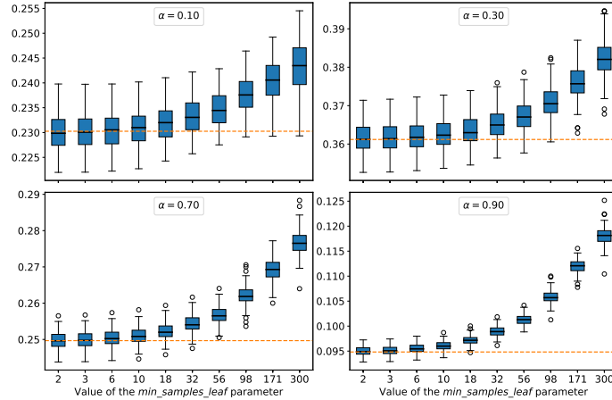
Figure 3: For several levels \alpha : distribution of \widehat{Q}_1^{3,o} , the estimation of the O term associated to the variable X_1 for different leaf sizes. The dotted orange line represents the true value on each plot.
