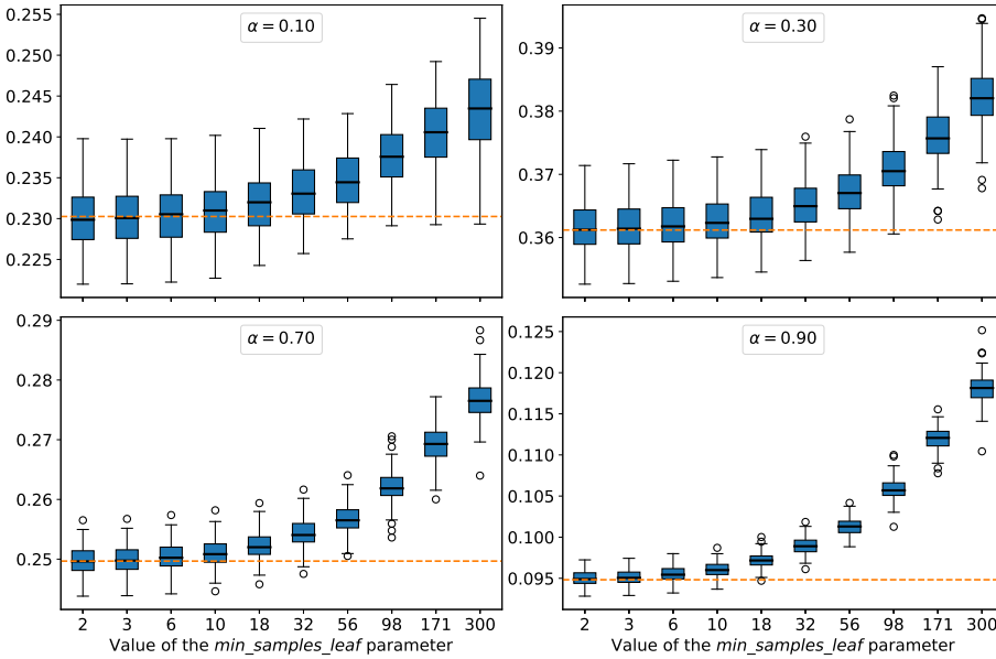
Figure 3: For several levels \alpha : distribution of \hat{Q}_1^{3,o} , the estimation of the O term associated to the variable X_1 for different leaf sizes. The dotted orange line represents the true value on each plot.
