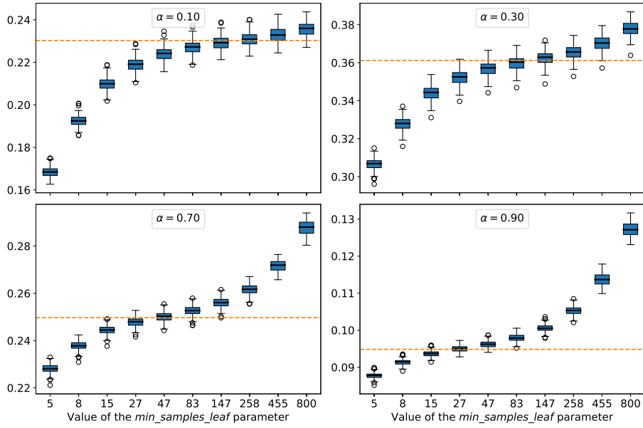
Figure 2: For several levels \alpha : distribution of \hat{Q}_1^{1,o} , the estimation of the O term associated to the variable X_1 for different leaf sizes. The dotted orange line represents the true value on each plot.
