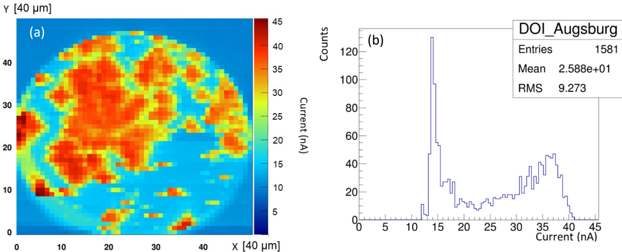
Figure 10 Histogram of the measured current normalized to \Phi_{32\text{mA}}(\text{ph}) = 1.79 \cdot 10^9 \text{ ph/s} (b) on the surface map (a) of a 0.5 \times 0.5 \text{ cm}^2 \times 300 \text{ }\mu\text{m} DOI detector from Augsburg University, biased at -300V.
