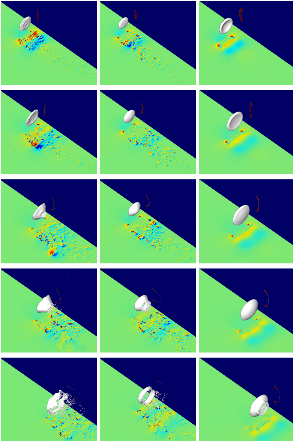
Figure 6: Isometric view, flow direction from top right to left bottom. Bottom plane colored by a_x (stream-wise acceleration component, range [-1.5;1.5] m/s 2 ), left plane colored by \tilde{c} function (range [0;1] ). t/t_c = 1.0, 1.64, 1.97, 2.14, 2.67 (top to bottom). Cases 1, 2 and 3 from left to right.
