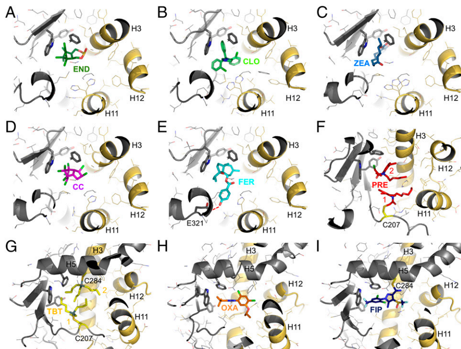
Fig. 2. Chemicals bind to PXR with varied binding mechanisms and pocket occupancies. (A–I) Close-up view of the LBP of PXR bound to the various test compounds. The chemicals (color code for carbon atoms as in Fig. 1A) and residues belonging to the aromatic cage (gray) are shown as sticks. Other residues are displayed as lines. Oxygen, nitrogen, sulfur, and chlorine atoms are colored in red, blue, yellow, and green, respectively. Residues and secondary structural elements discussed in the text are labeled.
