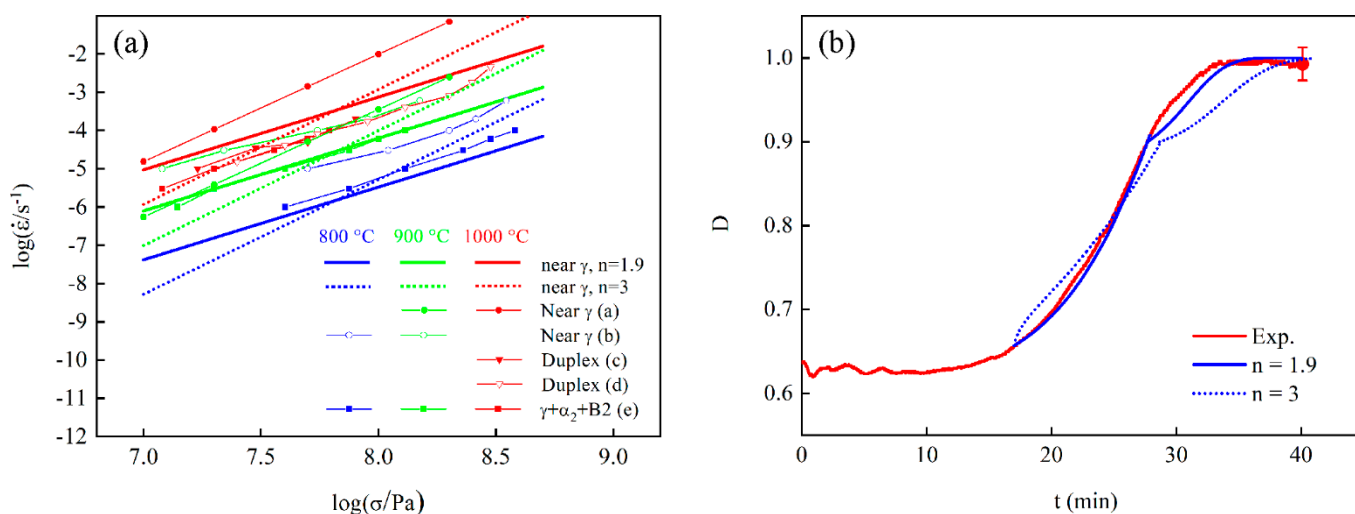
Figure 15. (a) Norton laws of a near \gamma TiAl alloy, taking n = 1.9 and n = 3 , the activation energy being identical ( Q = 308 kJ/mol). Comparison with literature data of alloys of similar near- \gamma and duplex microstructures ((a): [85], (b): [89], (c): [90], (d): [91], (e): [92]). (b) Densification curves of TiAl ( D : relative density, t : time) calculated using n = 1.9 [28], and n = 3 , compared with experiment.
