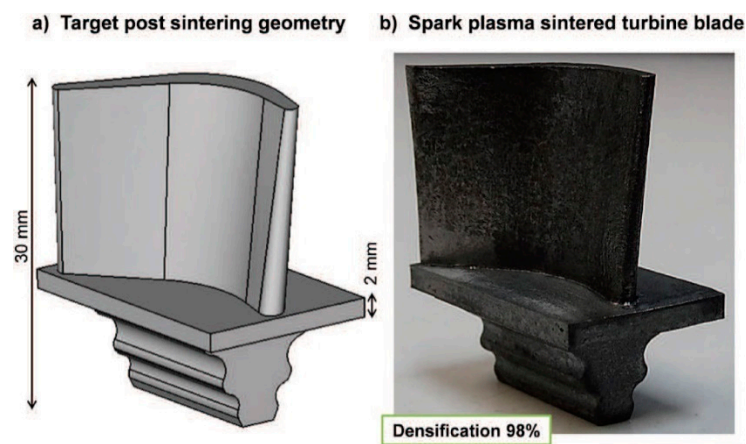
Figure 17. Example of turbine blade in CoNiCrAlY obtained by the deformed interfaces method. (a) Target shape. (b) Complex part obtained by SPS [97]. Reproduced with permission from Powder Technology , published by Elsevier, 2017.
