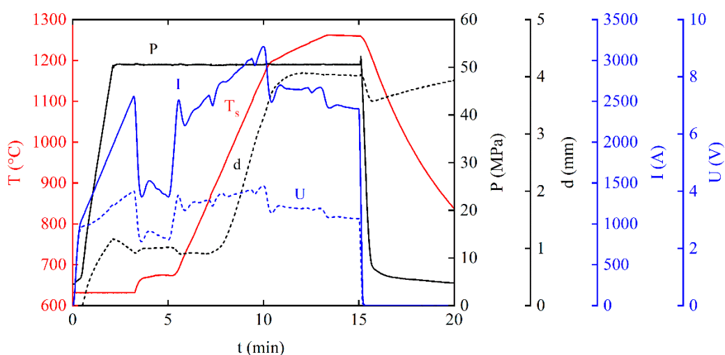
Figure 3. Evolution of the SPS parameters during the processing of a metallic TiAl alloy, in the case of a 36 mm sample ( T_s : corrected sample temperature, P: applied mechanical pressure, I: intensity, U: voltage and d: sample thickness reduction).
