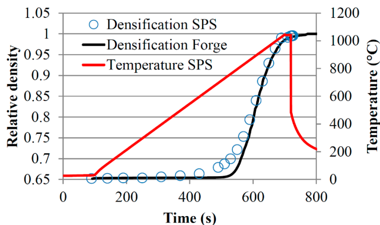
Figure 14. Densification kinetics by SPS of a TiAl alloy, compared with modeling by Forge software and continuum mechanics, using constitutive relations of bulk TiAl [85]. Reproduced with permission from Intermetallics , published by Elsevier, 2017.
