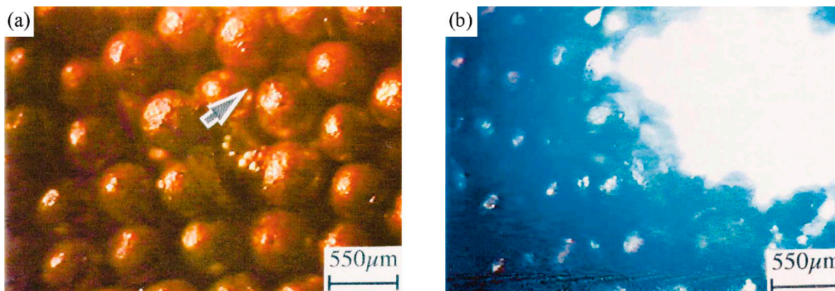
Figure 4. (a) Cu powder particles 550 \mu\text{m} in diameter. (b) Generation of an electric arc by a current pulse of 6700 \text{A}/\text{cm}^2 during 100 ms, at the location indicated by an arrow in Figure (a) [8]. Reproduced with permission from Materials Science and Engineering: A , published by Elsevier, 2003.
