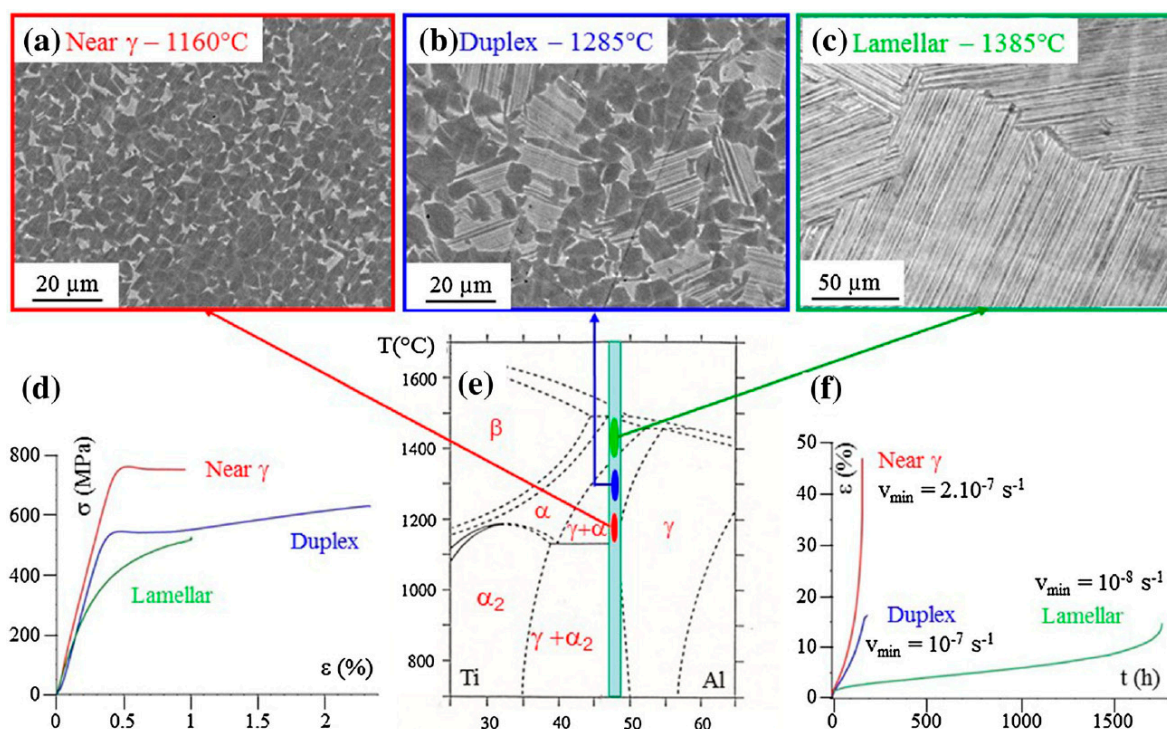
Figure 7. (a–c) Near \gamma , duplex, and lamellar microstructure of the Ti-Al 48 -Cr 2 -Nb 2 alloy obtained by elaboration by SPS, compared with the binary phase diagram of this alloy (e). Mechanical properties in tension at room temperature (d) and in creep (700 °C—300 MPa) (f) of the corresponding materials [30]. Reproduced with permission from Journal of the Minerals, Metals and Materials Society , published by Springer Nature, 2017.
