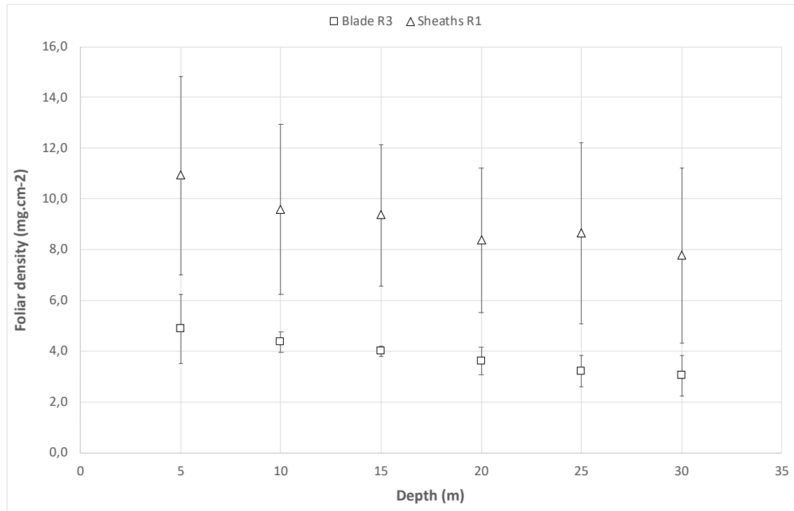
182 183 Figure 3: Blades and sheaths density (mean and confidence level 95%) according to depth. The high 184 values of the confidence interval are related to seasonal variations in leaf tissue density. 185
