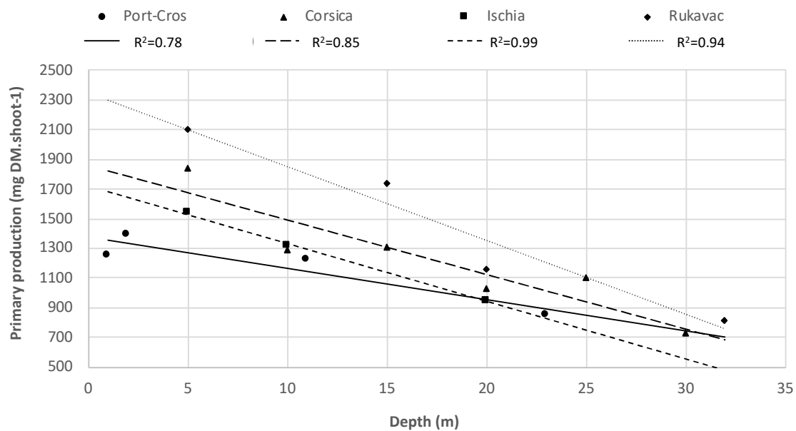
267 268 Figure 6: Annual primary production of P. oceanica (mg DM.shoot -1 ) according to depth and site, R 2 = 269 determination coefficient is reported (from Pergent-Martini et al. , 1994; Bakran-Petricioli & Schultz, 270 2010 and this study). 271
