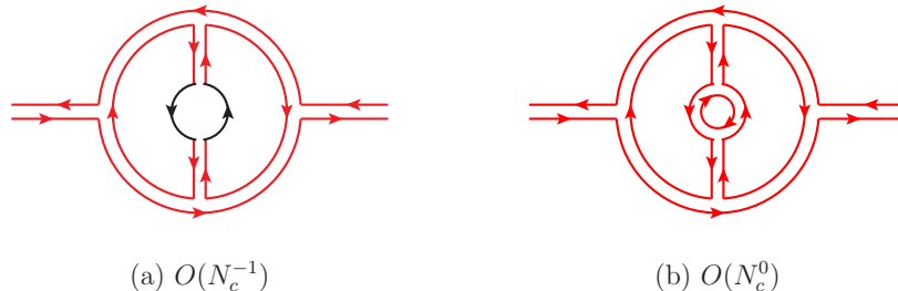
Figure 4: One-gluon exchange inside the gluon self-energy diagram: (a) including a quark loop; (b) including a gluon loop. The corresponding orders in large- N_c behavior are also indicated.
