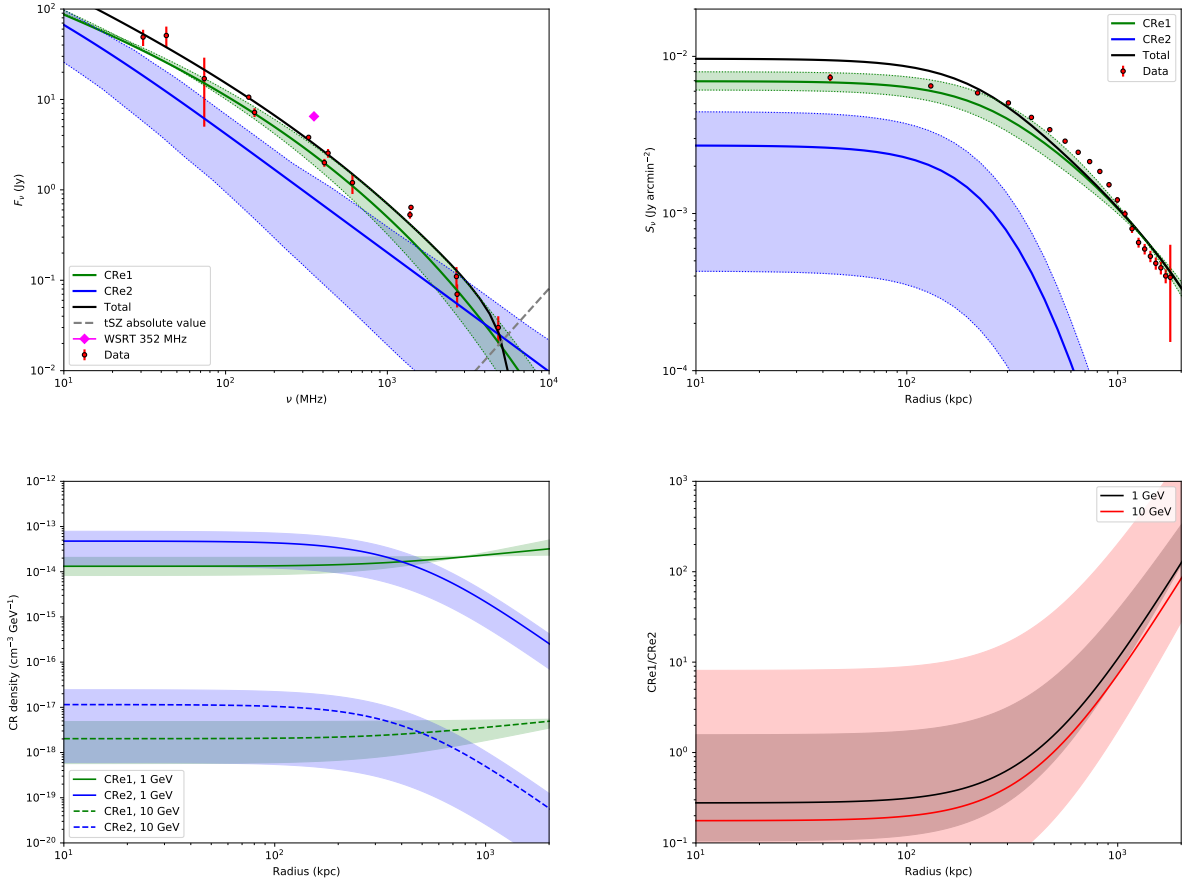
Fig. 12. Constraint on the CR populations in the case of scenario 1 (distinct \text{CRe}_1 and \text{CRe}_2 populations, no reacceleration). Top left: radio spectrum of Coma, as compiled from Pizzo (2010) and constraint from the reference CRp spatial model ( n_{\text{CRp}} \propto n_e^{1/2} ) and the reference \text{CRe}_1 spectral model (ExponentialCutoffPowerLaw). The measurement from the Brown & Rudnick (2011) data is also shown as the magenta diamond. The contribution from the \text{CRe}_2 is shown in blue together with its 68% confidence interval, and the remaining contribution from \text{CRe}_1 is shown in green. The sum of the two is given as the black line. The dashed gray line provide the expected amplitude of the tSZ signal. All fluxes are computed using cylindrical integration within R = 0.48 \times R_{500} = 629 \text{ kpc} \equiv 0.36 \text{ deg} . Top right: radio profile measured from the WSRT map at 352 GHz and comparison to the reference model. The contributions from \text{CRe}_2 and \text{CRe}_1 are as in the left panel. Bottom left: absolute number density distributions of \text{CRe}_1 and \text{CRe}_2 taken at 1 GeV and 10 GeV. Bottom right: ratio between the \text{CRe}_1 and \text{CRe}_2 number populations. We note that in the case of this figure, the confidence limits were computed using a resampling of only 100 parameters, and are thus not very accurate. We also stress that this figure depends on the magnetic field modeling (see Sect. 7.2 for discussions).
