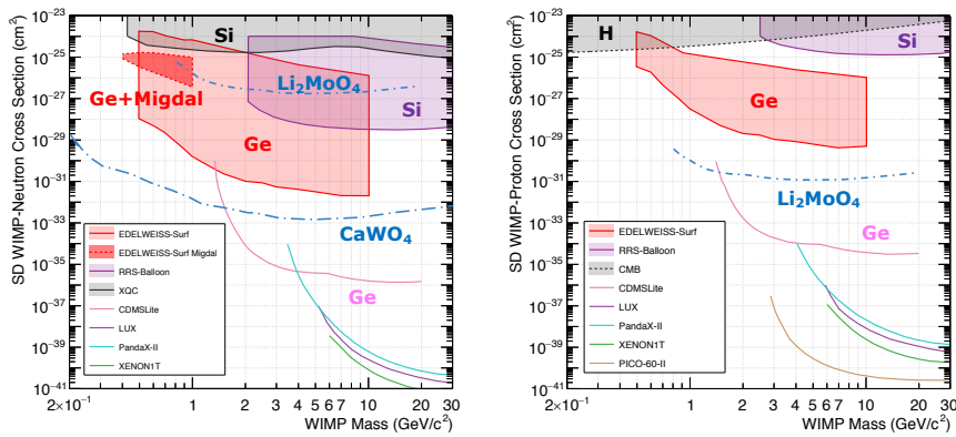
Figure 2: Constraints for spin-dependent interaction of SIMPs on neutrons (left panel) and protons (right panel), adapted from Ref. [14]. See references therein for the list of the different experiments, while the \text{CaWO}_4 and \text{Li}_2\text{MoO}_4 result are from Refs. [17] and [18], respectively. As in the previous figure, full contours correspond to calculations that include the full attenuation effects of Earth, atmosphere and experimental shielding. All lines correspond to limits that do not take these effect into account.
