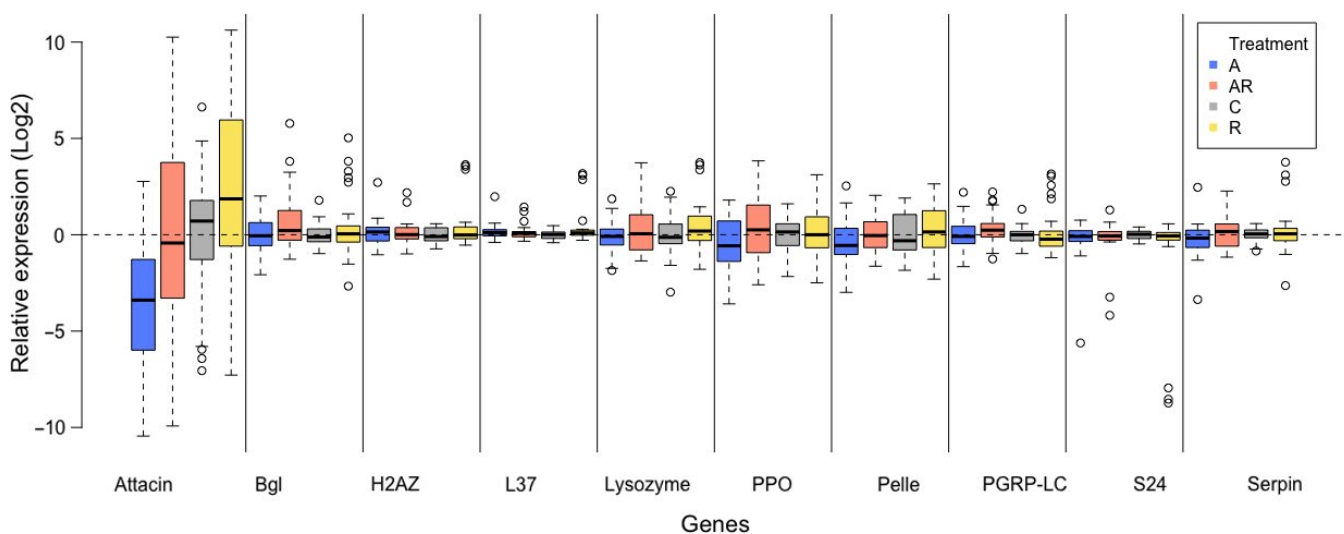
FIGURE 5 Effects of microbial depletion through antibiotic treatment on the expression levels of seven immune genes in prediapause larvae of the Glanville fritillary butterfly. Data include larvae from 12 larval families under four different treatments (A-Blue): antibiotic-treated, (AR-Orange): antibiotic-treated even during re-infected, (R-Yellow): antibiotic-treated followed by re-infection by L7 larval frass, and (C-Gray): controls. Expression levels of the three housekeeping genes ( H2AZ , L37 , and S24 ) are also shown
