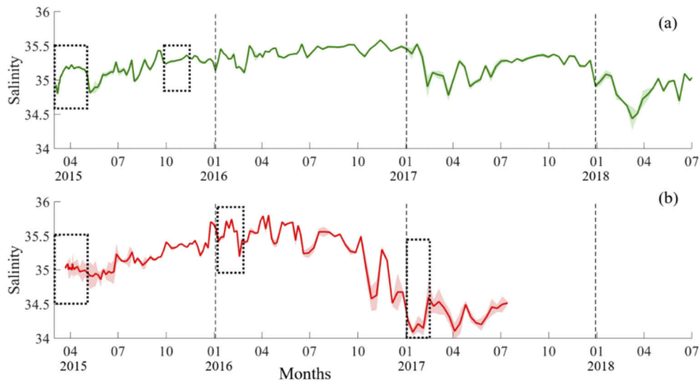
Fig. 5. Temporal variations of (a) the average salinity ( \pm sd) in the mixed layer for float F_A (green line) and (b) float F_B (red line). Black dashed frames show the “bloom periods” defined in the text.
