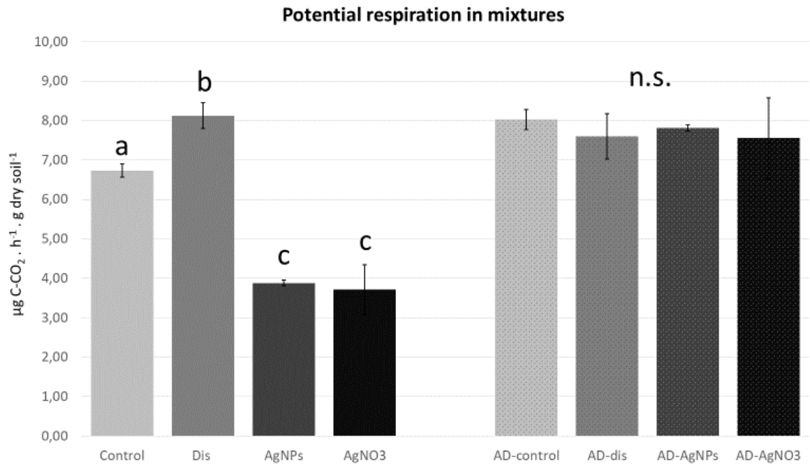
Figure 2: Potential carbon respiration of microbial communities in mixtures (µg C-CO 2 · h -1 · g -1 of dry soil). The letters indicate significant differences in respiration between the 4 treatments without sewage sludge. "n.s." indicates that there were no significant differences between the 4 treatments with sewage sludge.
