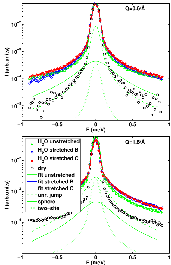
FIG. 8: (Color online) QENS data (symbols) from 100% RH H 2 O humid silk and dry silk, respectively. The thick solid lines are fits of eq. 9 simultaneously to all 5 Q -groups – out of which only two are shown – after convolution with the dry silk data which have been assumed as resolution function. The dashed lines indicate the contributions of unrestricted jump diffusion, the dash-dotted lines represent the two-site jump diffusion, and the thin solid lines mark the diffusion on a sphere, respectively, for the example of the unstretched 100% RH H 2 O-humid silk. All fit components are shown after convolution with the instrument resolution. The Q -dependence of eq. 9 has been imposed on the fit.
