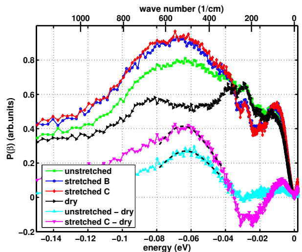
FIG. 6: (Color online) Q -integrated generalized frequency distribution calculated from the time-of-flight spectra on dry and humid samples at 100% RH \text{H}_2\text{O} , respectively. The dashed lines superimposed on the difference spectra "humid - dry" are indicative fits of a Gaussian line shape to determine the position of the maximum of the water librational peak. The capital letters in the legend refer to the positions on the stress strain curves marked in figure 2. The TOF-spectra have been normalized to equal total intensity for accurate comparison.
