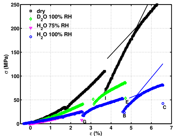
FIG. 2: (Color online) Stress-strain curves obtained in situ during the IN6 experiment using the apparatus depicted in figure 1 (humidities see legend, sample properties table I). TOF data have been recorded at the positions on the stress-strain curves marked by the capital letters and at \epsilon \approx 0 . The solid lines are linear fits to determine the mechanical moduli (see text).
