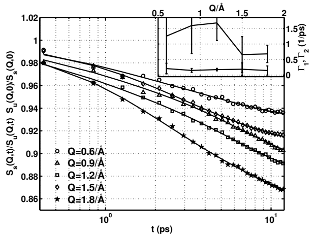
FIG. 7: Ratio of the intermediate scattering functions S_s(Q, t) from the 100% RH \text{H}_2\text{O} -humid silk stretched to position C (figure 2) and S_u(Q, t) from unstretched 100% RH \text{H}_2\text{O} -humid silk obtained from a Fourier transform of the data recorded on IN6 (symbols). The lines are fits of S_s(t)/S_u(t) = I_1 \exp(-\Gamma_1 t) + I_2 \exp(-\Gamma_2 t) . Inset: Fit results for \Gamma_1 and \Gamma_2 . The error bars denote 95% confidence limits of the fit.
