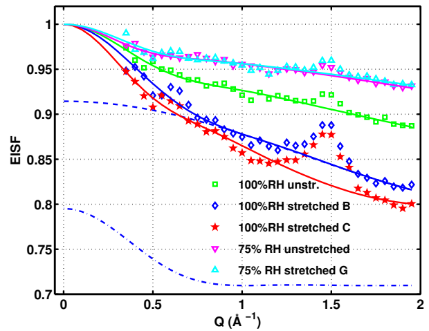
FIG. 5: (Color online) Elastic incoherent structure factors (symbols) of H_2O -humid silk (100% RH and 75% RH, respectively), calculated from S(Q, \omega) -data grouped in Q . The solid lines denote fits according to eq. 2. The dashed and dash-dotted lines indicate the two-site jump and diffusion inside a sphere contributions, respectively, for the silk stretched to position B in figure 2. The poly-alanine peak near 1.4 \text{ \AA}^{-1} (figure 4) has been excluded from the fit. In eq. 3, p = 0.5 has been fixed. The humid silk EISFs have been normalized by the dry silk EISF. The fit parameters are summarized in table II.
