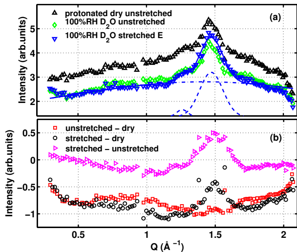
FIG. 4: (Color online) (a) Diffraction patterns recorded on IN6 on dry and 100% RH D_2O -humid silk (symbols). The scattering intensities have been normalized taking into account the different illuminated masses. The label "E" refers to the stress-strain curve (Fig. 2). The solid line is a fit of a sum of three Gaussians, denoted by dashed and dash-dotted lines, respectively, to the D_2O -humid stretched silk. (b) Difference patterns from (a) as specified in the legend. The labels "stretched" and "unstretched" both denote 100% D_2O -humid silk.
