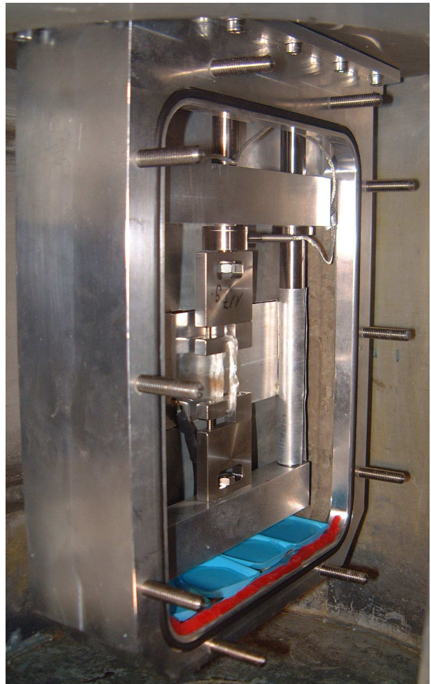
FIG. 1: (Color online) Photograph of a silk sample (white fiber bundle in the center of the image) inside the humidity chamber for in situ tensile testing mounted inside the sample bay of the time-of-flight spectrometer IN6. The chamber is shown with the front cover removed. The force sensor is visible as a cylindrical metal structure on the upper center of the photograph with the signal cable arriving from the right. The neutron beam impinges on the sample horizontally, arriving from the right edge of the photograph. The blue plastic troughs at the bottom of the chamber contain pure water or saturated salt solutions, respectively, to define the humidity inside the chamber. The edge-to-edge distance between the steel hooks holding the fiber bundle is 3 cm.
