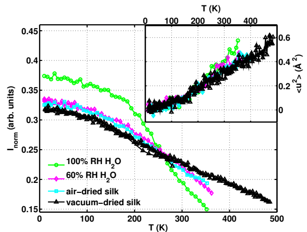
FIG. 3: (Color online) Elastic scattering intensities recorded on IN10 within the 1\mu\text{eV} resolution window, integrated over all detectors. All data have been taken on the same silk sample, and the differences in the intensities at the lowest temperature are therefore a measure of the water contents. Inset: Mean-squared displacements \langle u^2 \rangle calculated from the Q -dependence of the intensities I(Q) according to I(Q) \propto \exp(-\frac{1}{3}\langle u^2 \rangle Q^2) .
