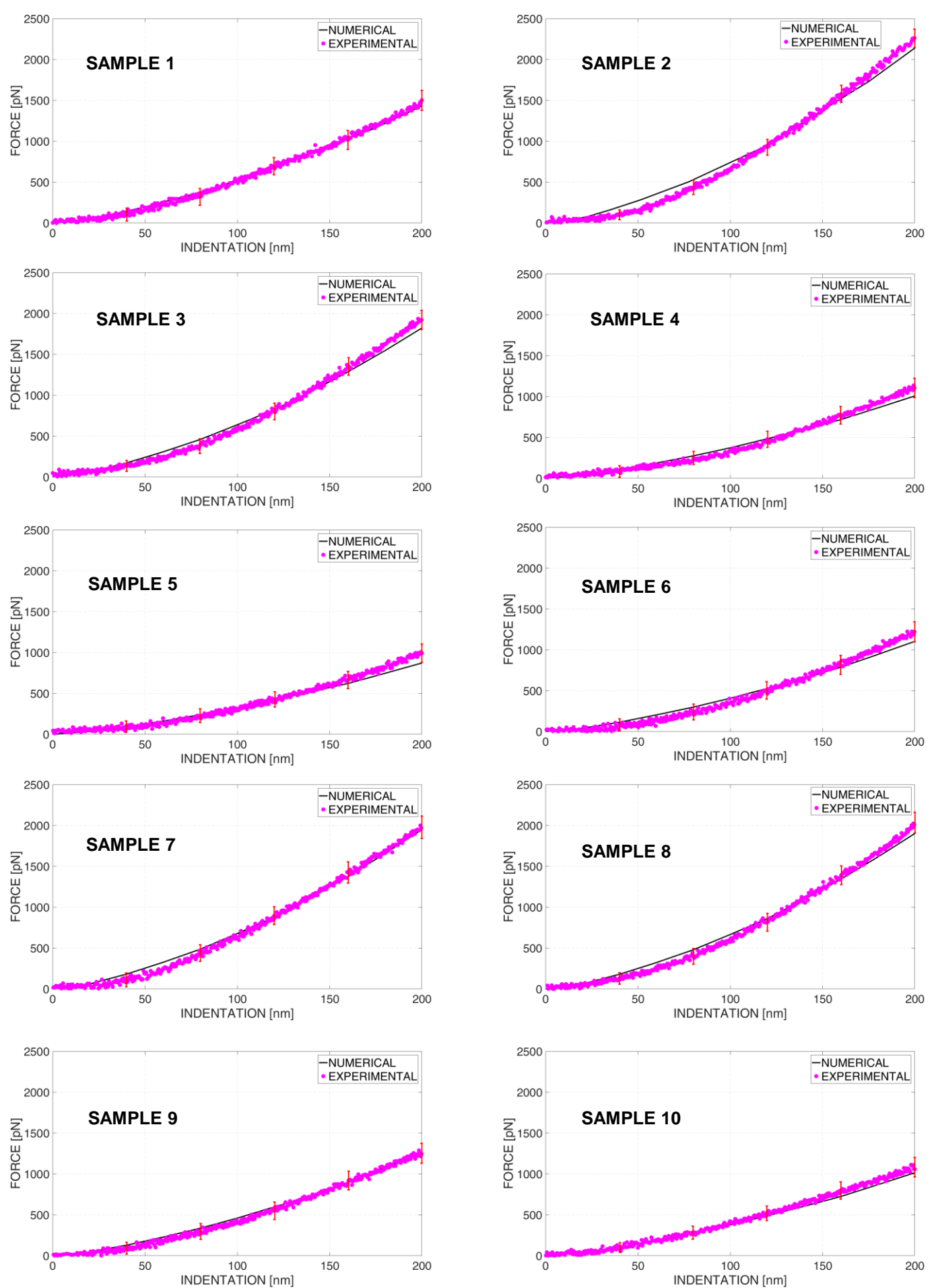
Fig. 9. Experimental force-indentation curves registered for the ten stem cell samples and related numerical curves predicted via the optimization algorithm. Error bars were superimposed to the average experimental force-indentation curves to show the dispersion of data at different indentation depths.
