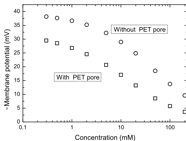
Figure 4. Simulated -membrane potential (mV) vs concentration (mM) with and without PET support. Graphene pore radius = 1.5 \text{ nm} ; graphene surface potential = -85 \text{ mV} .
