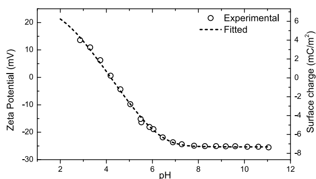
Figure 3. Zeta potential (from streaming potential measurements) fitted with the 1-pK model. The surface charge density derived from the zeta potential is plotted in the right axis.
