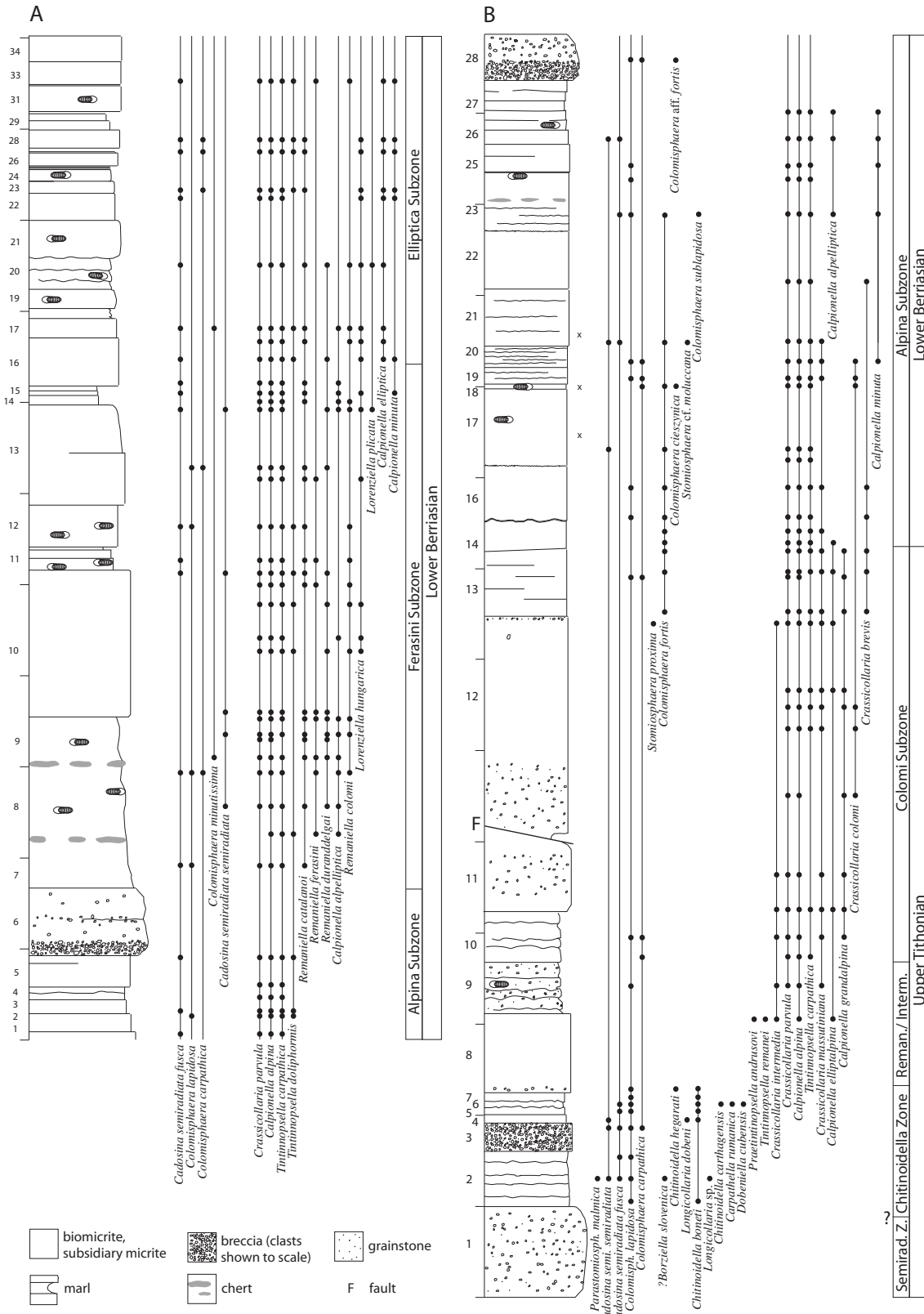
Fig. 5. The Tré Marroua lower (B) and lower-upper (A) sections
