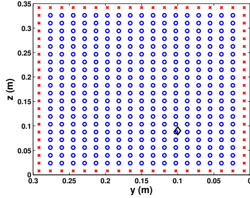
Figure 10: Definition of the identification regions - (○) region 1 (Point force), (×) region 2 (Boundary forces) and (◇) location of the point force
