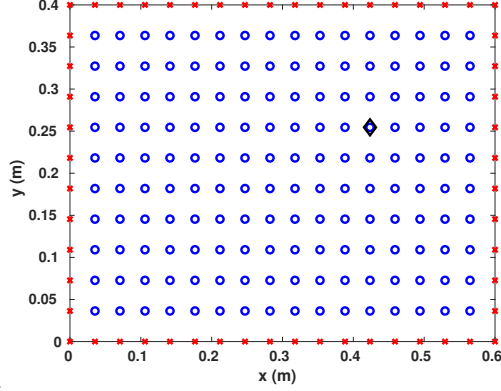
Figure 2: Definition of the identification regions - (○) region 1 (Point force), (×) region 2 (Reaction forces) and (◇) location of the point force
