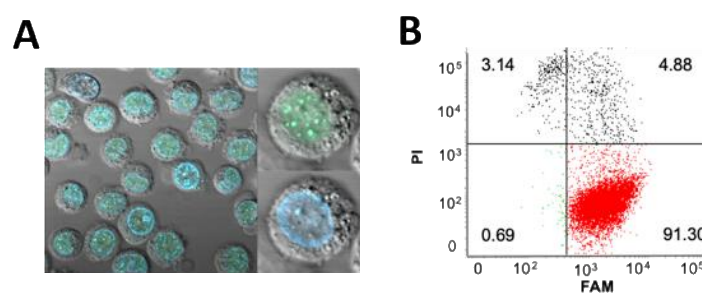
Figure S33 (A) Confocal microscopy image and (B) double-staining (PI/FAM) FCM analysis post temperature resolved in-cell NMR spectra acquisition of cells cotransfected with the (FAM)-T121-6. For meaning of colors and description of quadrants in the confocal image and FCM plot see legend of Figure S32 .
