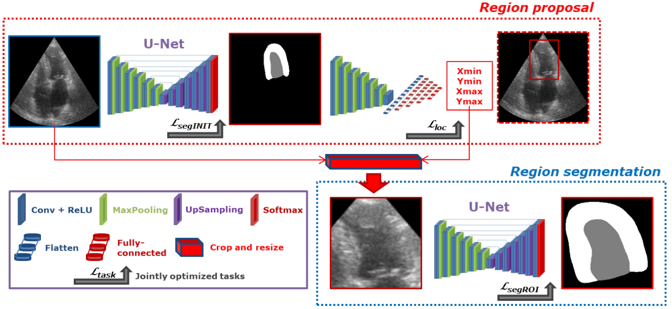
Fig. 1. Illustration of the LU-Net pipeline with the U-L2-mu localization network introduced in Sec. II-B2. The two U-Nets are independent.
