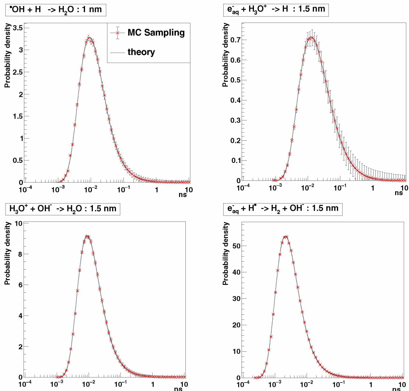
FIG. 1. Sampled times to reaction from the probability densities of reactions (“theory”) using the IRT method presented in this work. \text{H}^\bullet + \text{OH}^\bullet \rightarrow \text{H}_2\text{O} (initial distance of reactants 1.0 nm, partially diffusion-controlled), \text{H}_3\text{O}^+ + \text{e}_{\text{aq}}^- \rightarrow \text{H}^\bullet + \text{H}_2\text{O} (initial distance of reactants 1.5 nm, partially diffusion-controlled), \text{H}_3\text{O}^+ + \text{OH}^- \rightarrow 2 \text{H}_2\text{O} (initial distance of reactants 1.5 nm, totally diffusion-controlled), \text{H}^\bullet + \text{e}_{\text{aq}}^- + \text{H}_2\text{O} \rightarrow \text{OH}^- + \text{H}_2 (initial distance of reactants 1.5 nm, totally diffusion-controlled). [Color figure can be viewed at wileyonlinelibrary.com ]
