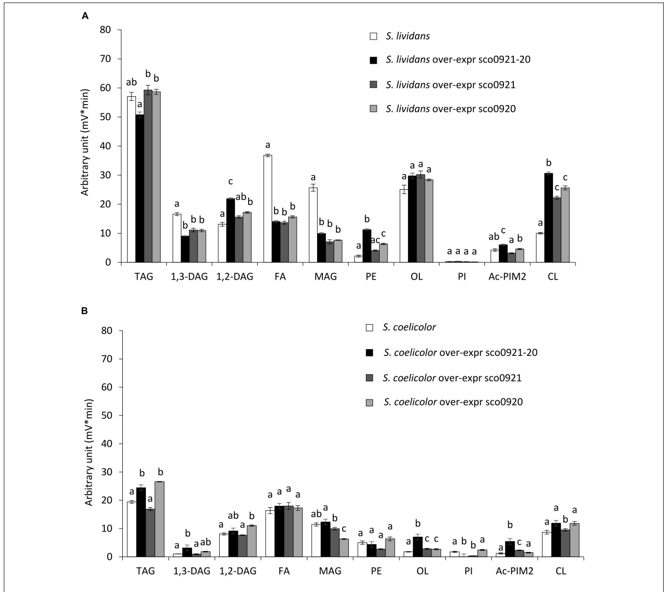
FIGURE 5 | LC/Corona-CAD analysis of the total lipid content of wt strains S. lividans TK24 and S. coelicolor M145 and of these strains over-expressing under the control of the strong ermE* promoter, the sco0921-20 operon or sco0921 or sco0920 alone. The strains were grown for 72 h at 28°C on solid R2YE medium with glucose (50 mM) as the main carbon source and containing 1mM phosphate (Pi limitation). (A) LC/Corona-CAD analysis of total lipid content of S. lividans TK24 (white histograms), S. lividans TK24 over-expressing the sco0921-20 operon (black histograms), S. lividans TK24 over-expressing sco0921 (dark gray histograms) and S. lividans TK24 over-expressing sco0920 (light gray histograms). (B) LC/Corona-CAD analysis of the total lipid content of S. coelicolor M145 (white histograms), S. coelicolor M145 over-expressing the sco0921-20 operon (black histograms), S. coelicolor M145 containing an extra copy of sco0921 (dark gray histograms) and S. coelicolor M145 containing an extra copy of sco0920 (light gray histograms). TAG, triacylglycerol; DAG, diacylglycerol (1,2 or 1,3); FA, fatty acids; MAG, monoacylglycerol; PE, phosphatidylethanolamine; OL, ornithine lipids; PI, phosphatidylinositol; Ac-PIM2, acetylated phosphatidylinositol mannoside 2; CL, cardiolipid. Means values are shown as histograms with error bars representing standard error. Means sharing a letter are not significantly different ( P > 0.05 ; Tukey-adjusted comparisons).
