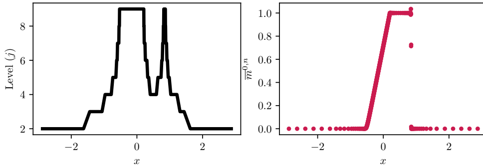
FIG. 5. Example of solution of the D_1Q_2 for the Test IV, considering n = 358 , s^1 = 1.5 and \epsilon = 10^{-4} . On the left, levels of the computational mesh. On the right, solution on the leaves of the tree.
