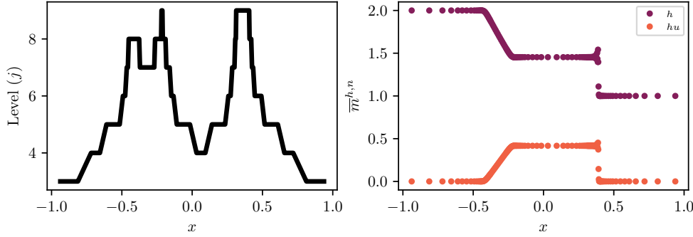
FIG. 6. Example of solution of the D_1 Q_5 for the shallow water problem with n = 300 , s^2 = 1.6 and \epsilon = 10^{-4} . On the left, levels of the computational mesh. On the right, solution on the leaves of the tree.
