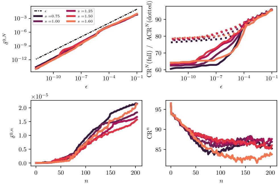
FIG. 7. D_1 Q_3 for the shallow water system with Riemann initial datum. The dot-dashed line gives the reference \delta^{0,N} = \epsilon . For the sake of avoiding redundancy, we present only one moment. s is a shorthand for s^2 .
