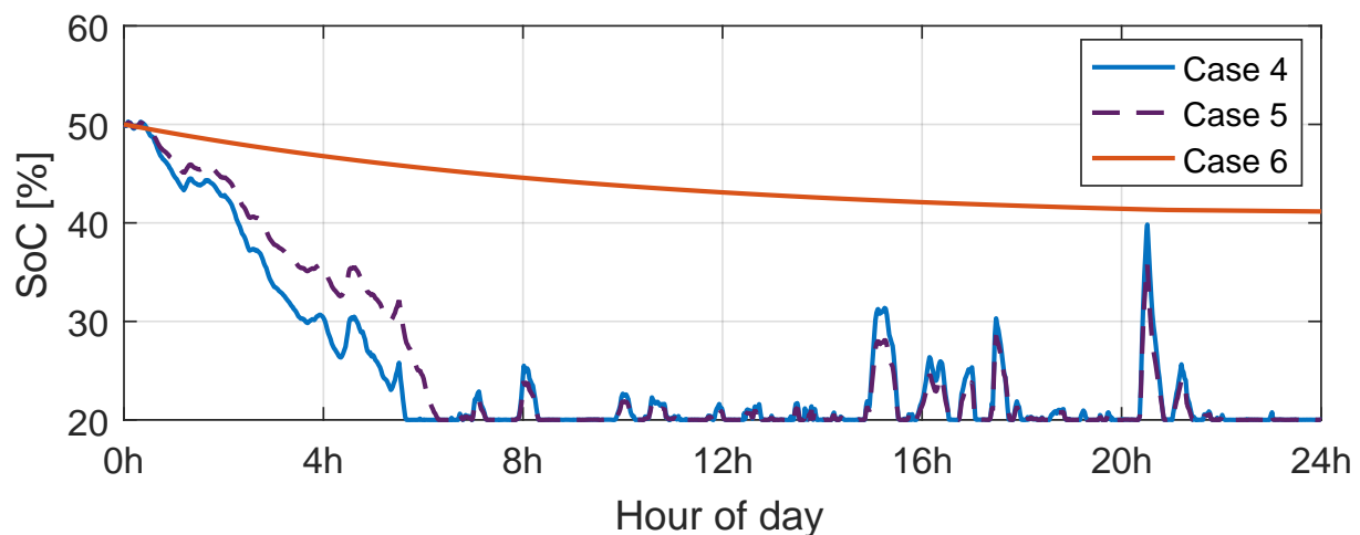
Figure 29. Strategy 2: SoC signals with Case 4: \lambda_1 = 100 , \lambda_2 = 0 , Case 5: \lambda_1 = \lambda_2 = 50 , and Case 6: \lambda_1 = 0 , \lambda_2 = 100 . Initial SoC of 50% and P_{SCHED} with maximum \pm 30\% error.
