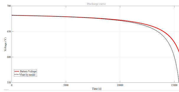
Figure 7. Battery discharge curves: red line, SimPowerSystems battery, and implemented nonlinear Trebley model in gray.
