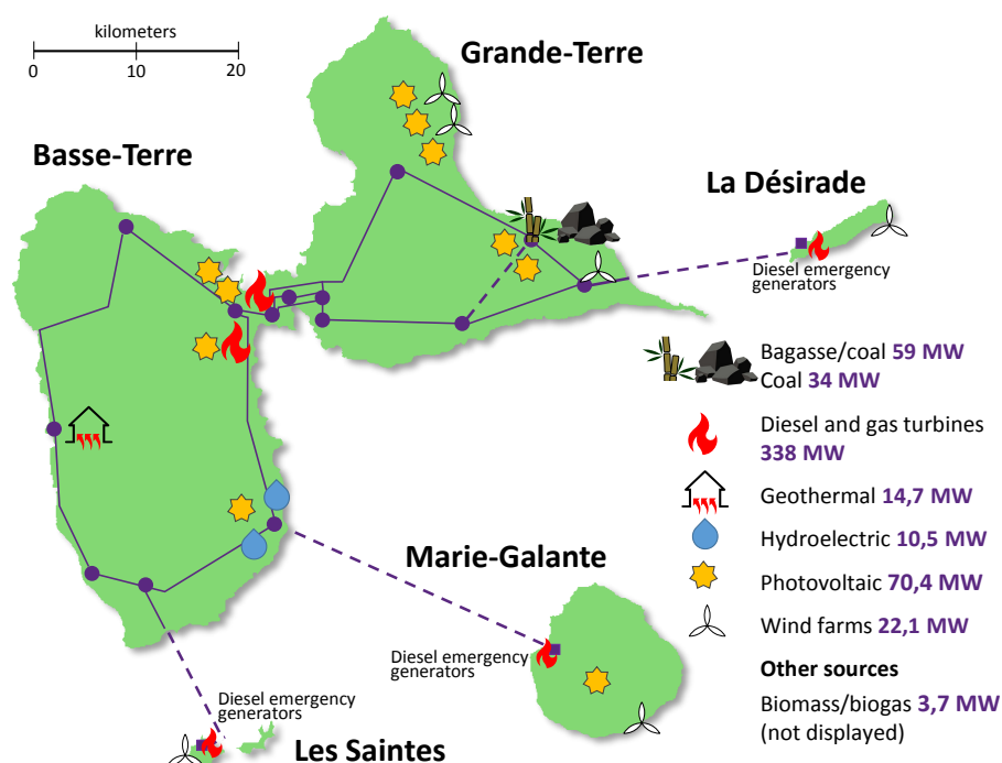
Figure 1. Available power in Guadeloupe's power grid by type of primary energy in 2018.
