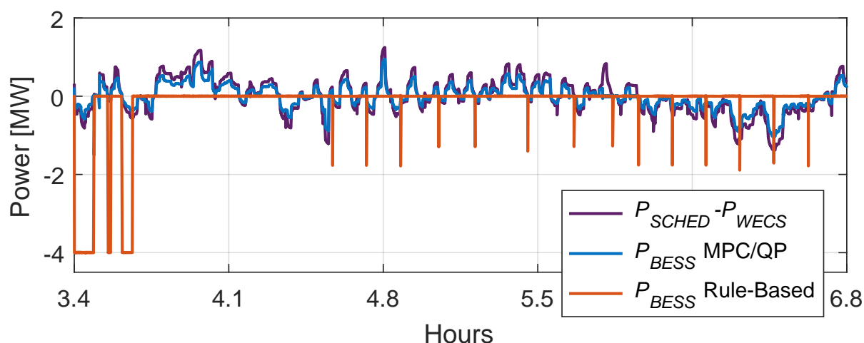
Figure 31. Close view of BESS power using MPC/QP and rule-based algorithms in PowerFactory.
