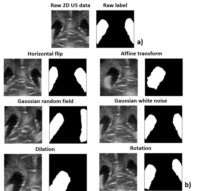
Fig. 1. US data and associated label without (a) and with artificial data augmentation (b).
