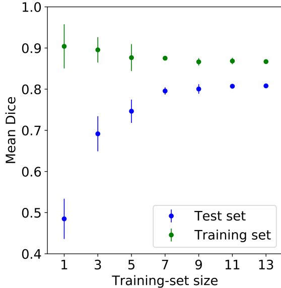
Fig. 2. Mean dice calculated over the training set and the test set as a function of the training-set size (without data augmentation).
