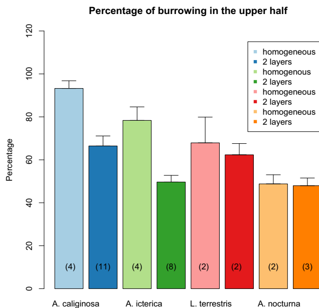
Fig. 2 Percentage of the burrow system found in the upper half (0–15 cm) of the repacked soil cores depending on the earthworm species and the soils used (a homogeneous soil layer or two layers). Soil cores were either (i) homogeneously filled with a soil with a higher content in organic matter (4%) or (ii) filled in two halves with the lower half containing a soil less rich in organic matter (2%) and the upper part was filled with a soil rich in organic matter (4%). The number between brackets indicated the number of earthworm per soil core
