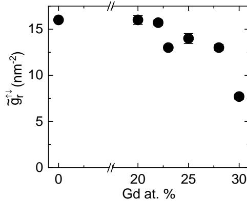
FIG. 11. Composition dependence of the renormalized reflected mixing conductance \tilde{g}_r^{\uparrow\downarrow} at the Cu/ Co 100-x Gd x interface with the Co 100-x Gd x spin sink thickness d \gg \lambda_{dp} .
