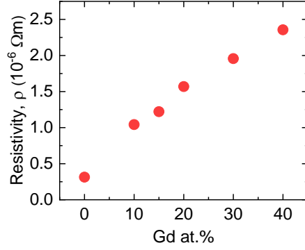
FIG. 13. Resistivity \rho with varying Gd at.% for SiO x (thermally oxidized)/Co 100-x Gd x (10)/TiO x (3) (unit: nm). The resistivities of intermediate compositions between x = 20 and 30 are derived via linear interpolation.
