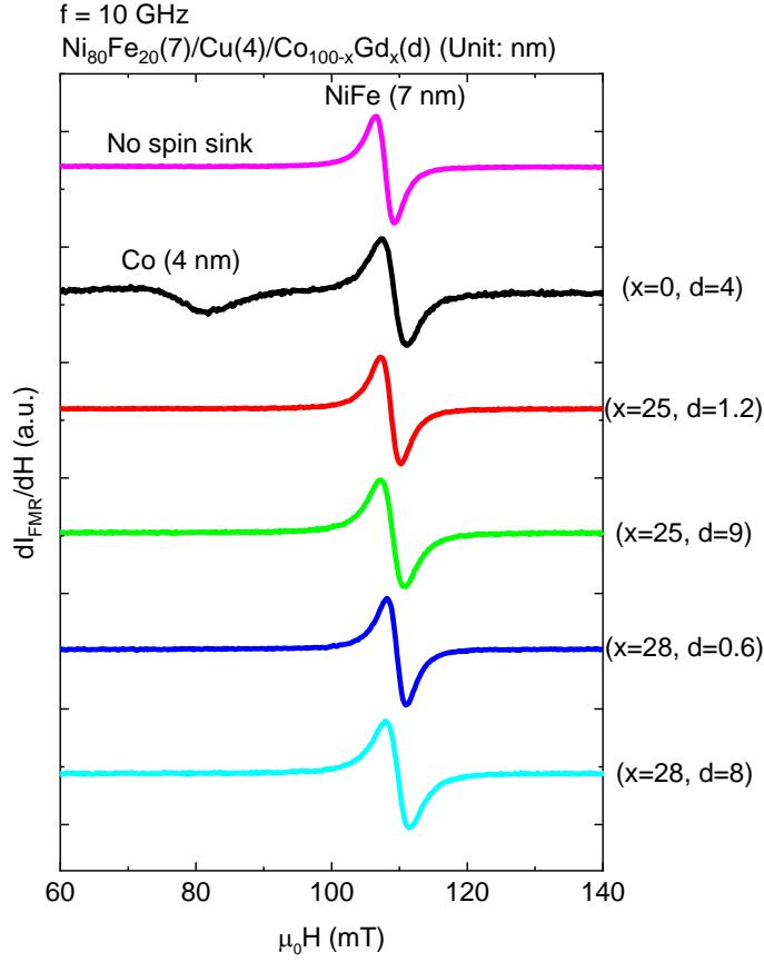
FIG. 10. FMR spectra for \text{Ni}_{80}\text{Fe}_{20} (7 nm)/Cu (4 nm)/ \text{Co}_{100-x}\text{Gd}_x ( d nm) with no spin sink (magenta) and with spin sink layer of pure Co (black), Gd 25% (red and green) and Gd 28% (blue and light blue). NiFe and Co exhibit well-separated FMR. The different thicknesses for Gd 25 and 28% was selected to show two different transport regimes, i.e., below/above the \lambda_{dp} found from Fig. 6 in the main text. No FMR signal attributable to \text{Co}_{100-x}\text{Gd}_x in our samples ( 20 \leq x \leq 30 ) is detected.
