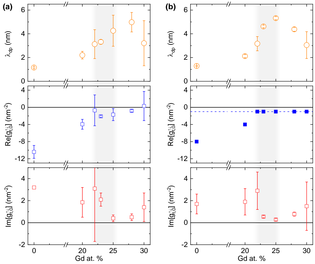
FIG. 16. Comparison of modeling results with (a) free \text{Re}[g_{t,0}^{\uparrow\downarrow}] and (b) fixed \text{Re}[g_{t,0}^{\uparrow\downarrow}] . The shaded region indicates the window of composition corresponding to magnetic compensation.
