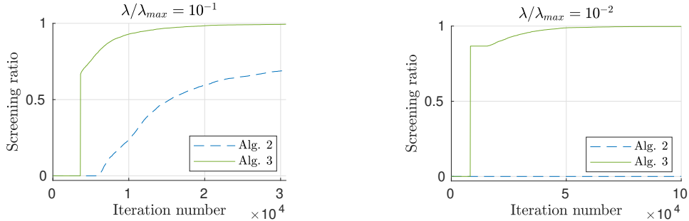
(b) Screening ratio against iterations for fixed regularization \lambda/\lambda_{\max} = 10^{-1} (left) and \lambda/\lambda_{\max} = 10^{-2} (right), corresponding to the dotted slices in Figure 4a.
