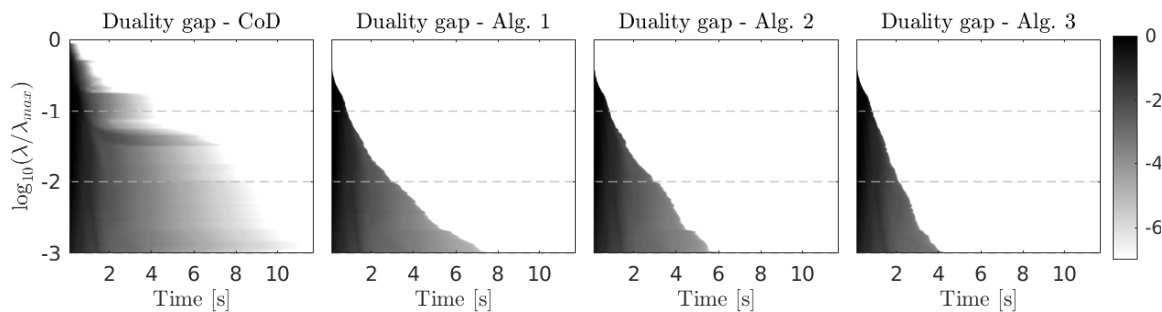
(c) Convergence rate (duality gap) against execution time for \lambda/\lambda_{\max} \in [10^{-1}, 10^{-3}] (the lighter, the closer to convergence). Left to right: Coordinate Descent solver alone and in Algorithms 1 to 3.
