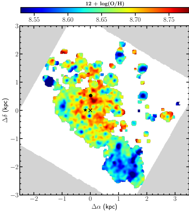
Fig. 9. Distribution of the metallicity derived using the calibration of Curti et al. (2017) using the H \beta , [OIII], [NII], and H \alpha lines with an S/N > 5 . The black cross, star, and filled circle show the position of the photometric, stellar, and gas kinematical centres, respectively.
