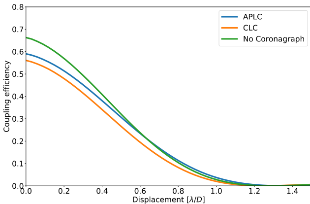
Fig. B.1. Coupling efficiency as a function of displacement between the PSF core and the Gaussian mode of the fiber. Evaluated at a wavelength of 1.6\mu\text{m} for three different coronagraph options.
