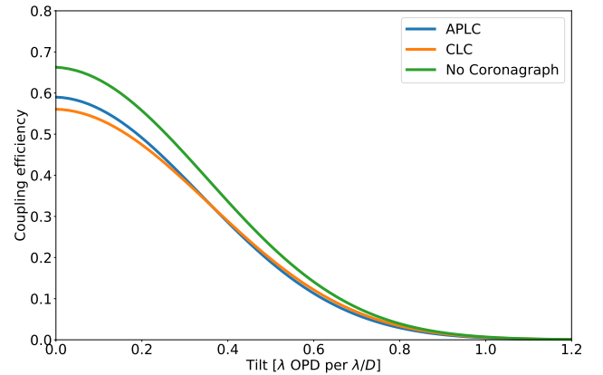
Fig. B.2. Coupling efficiency as a function of focal plane wavefront tilt between the PSF and the Gaussian mode of the fiber. Evaluated at a wavelength of 1.6\mu\text{m} for three different coronagraph options. A tilt of one \lambda of optical path difference (OPD) per \lambda/D equals \tan^{-1}(1/3.5) = 15.95^\circ .
