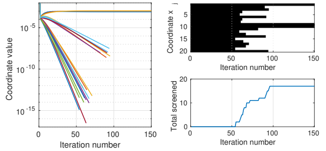
Fig. 1: Screening behavior with MU solver. Problem parameters: m = 10 , n = 20 , \lambda = 10^{-3} \lambda_{\max} . Left: each line is a coordinate x_j , the line stops when the coordinate is screened. Top: rows are coordinates which turn white when screened. Bottom: Total number of screened coordinates per iteration.
