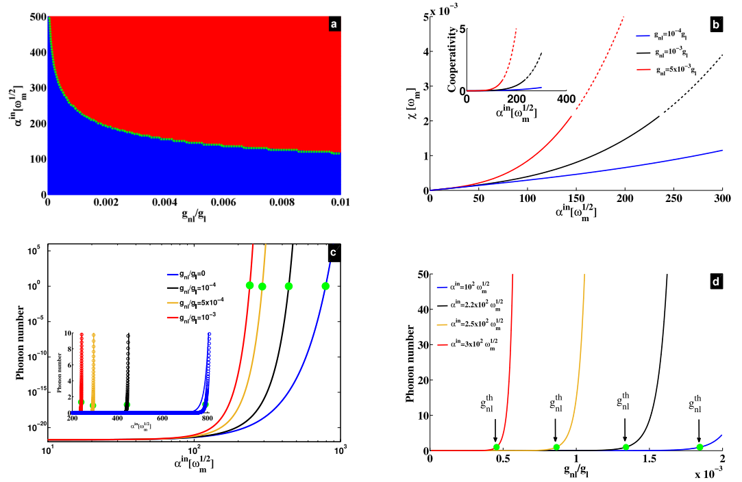
Figure 1. (a) Stability diagram. Blue (red) color is stable (unstable). The green dashed curve shows the border between stable and unstable regions, and corresponds to the lasing threshold C = 1 , with the cooperativity C = 4\chi^2/(\gamma_m\kappa) . (b) Effective coupling \chi versus \alpha^{in} for different values of g_{nl} . Full (dashed) curves are stable (unstable). The inset shows the cooperativity C versus \alpha^{in} , for the corresponding values of g_{nl} . (c) Phonon number versus \alpha^{in} in log-log scale, showing the fast increase near the thresholds. The inset displays the same figure in the linear scale, where full curves are from numerical simulation of classical version of Eq. (2), while the dotted lines represent the analytical approximation from N \sim \exp(-\gamma_{eff}t) . (d) Analytical (approximated) phonon number versus g_{nl} . In (c,d), the different lasing thresholds ( C = 1 ) are indicated by the green dots, namely \alpha^{in,th} and g_{nl}^{th} for the input field and the nonlinear coefficient, respectively. The used parameters are 20,23 , \gamma_m = 10^{-3}\omega_m , \kappa = 2 \times 10^{-2}\omega_m , g_l = 2 \times 10^{-5}\omega_m , and \Delta_0 = \omega_m .
