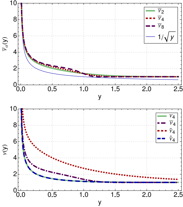
Figure 1. Representation of different MOND transition functions v (see equations 5 for their expression).
