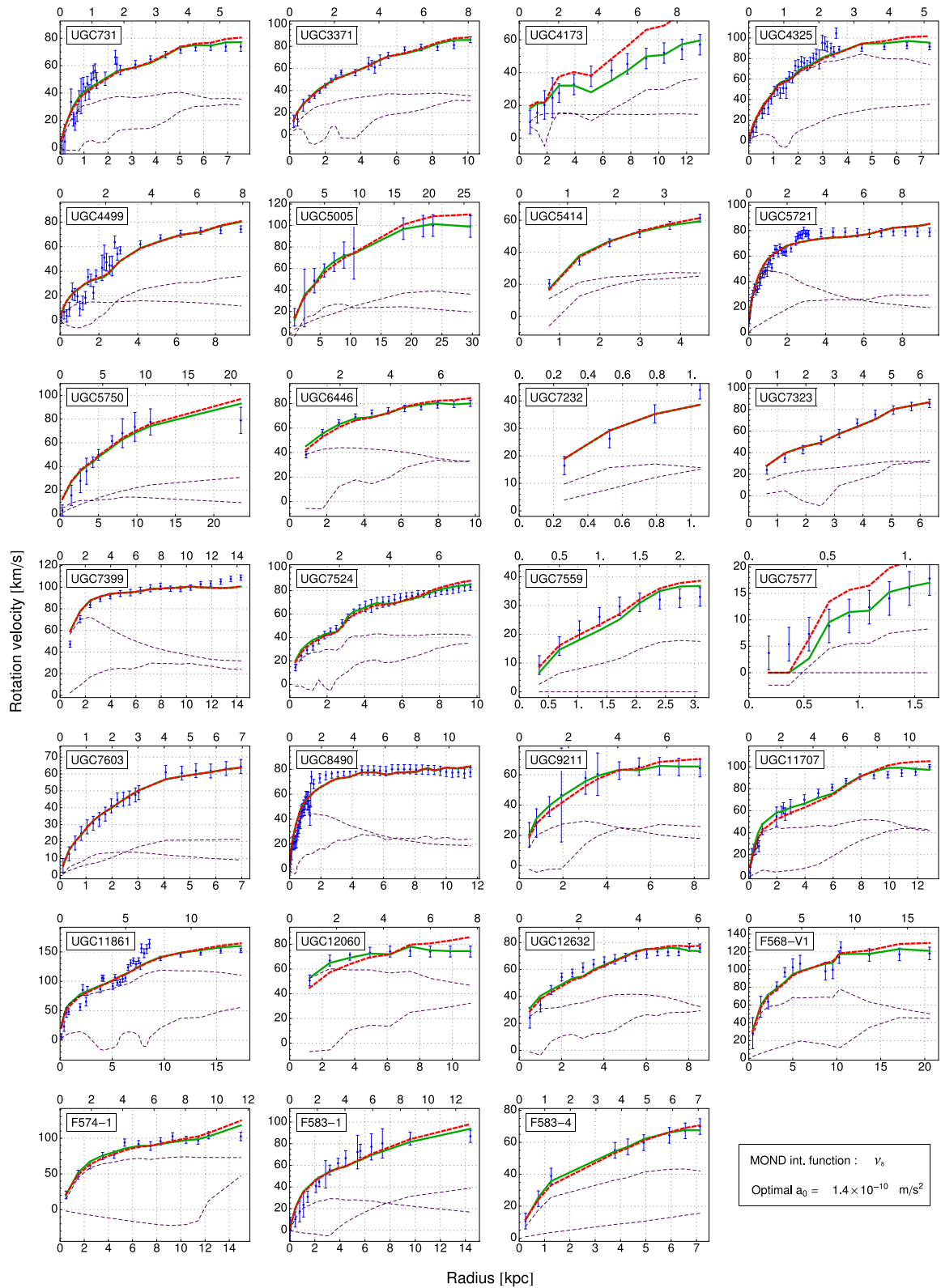
Figure A1. Results of the fits using the MOND transition function v_\phi for the optimal value a_0 = 1.4 \times 10^{-10} \text{ m s}^{-2} . The dashed (red) thick lines represent the optimal fit without any EFE; the thick (green) solid line represents the optimal fit with EFE; the thin solid line represents Newtonian the contributions of the stars; and the thin dashed line represents the gas contribution. Since the optimal fits with and without EFE do not necessarily produce the same distance scale factor, the radial scales may not be the same. On the top of the plots we mention the radial scale obtained without EFE, at the bottom of the plots we mention the radial scale obtained with EFE.
