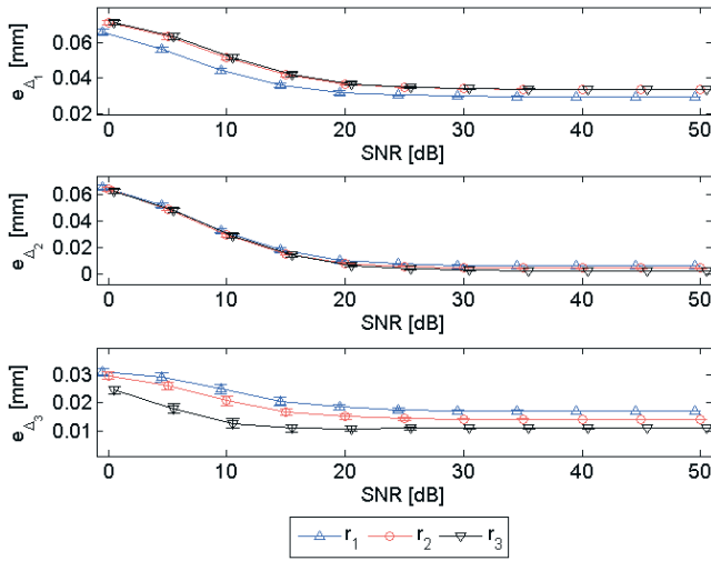
Fig. 3. Comparison of mean and standard deviation values of the absolute error between true and estimated displacement vectors using phase vector components. Absolute errors for \Delta_1, \Delta_2, \Delta_3 are displayed respectively from top to bottom.
