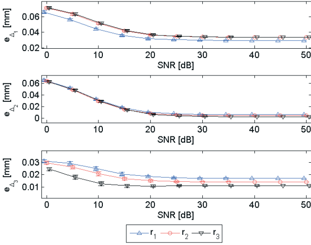
Fig. 3. Comparison of mean and standard deviation values of the absolute error between true and estimated displacement vectors using phase vector components. Absolute errors for \Delta_1 , \Delta_2 , \Delta_3 are displayed respectively from top to bottom.
