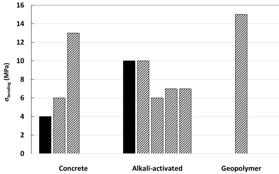
Figure 7: bending values in the literature for concretes (Wolf et al. 2019, Bos et al. 2019, Le et al. 2012), alkali-activated materials (Paul et al. 2018, Bong et al 2019, Al-Qutaifi et al 2018, Panda et al. 2017, Korniejenko et al. 2019) and geopolymers (values from this study) for ■ binders and ▨ composites shaped by robocasting.
