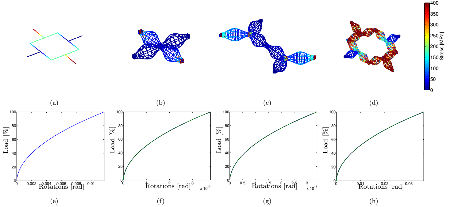
Figure B.17: Stresses and load-displacement curves considering torsional behavior for (a, e) non-hierarchical, (b, f) square hierarchical, (c, g) hexagonal hierarchical, and (d, h) hierarchical square structures.
