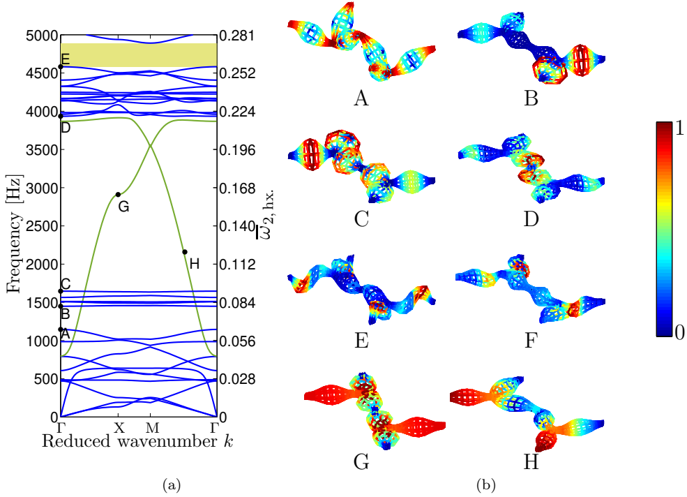
Figure 7: Band diagram and wave mode shapes (colored according to the magnitude of normalized displacements) from the two-dimensional hexagonal lattice obtained using the structure from Figure 2e. (a) Band diagram with interesting wave mode shapes indicated using letters A – H. (b) Wave mode shapes A, B, C, and D are at the contour of a region that has the potential to attenuate waves, even though it is not a complete BG, and wave modes G and H are used to illustrate typical modes; wave mode shapes E and F denote full BG edges between 4582 Hz and 4891 Hz.
