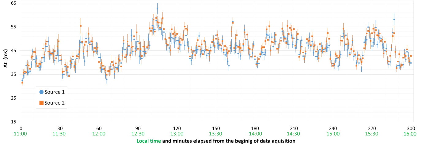
Figure 2. Temporal evolution of the coherence time ( \Delta t ) for each source with its standard deviation (October 30 th , 2015).
