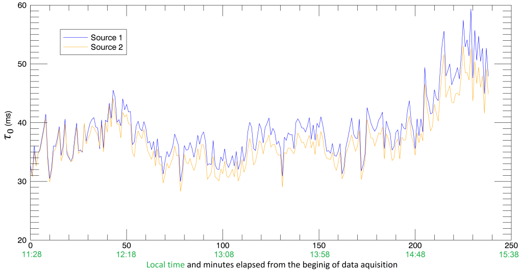
Figure 3. Temporal evolution of the coherence time of the phase \tau_0 for each source (October 19 th , 2015).
