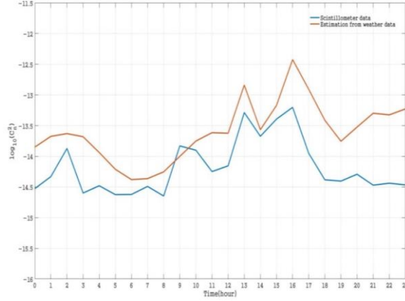
Figure 5: Comparison of estimated and measured C_n^2 values
