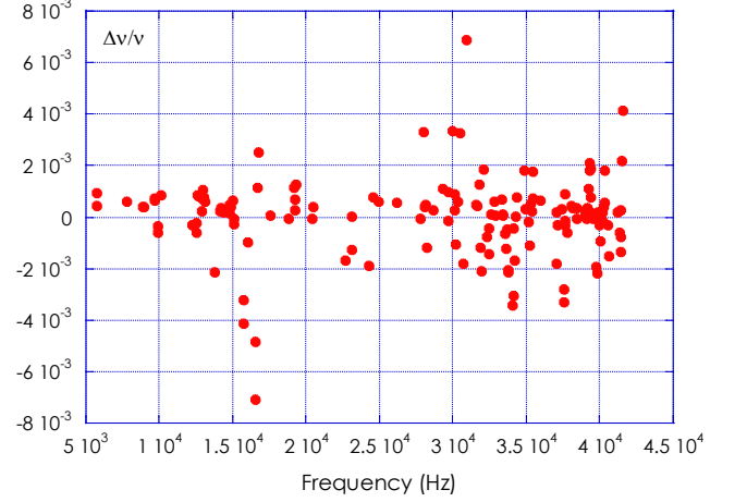
FIG. 3. Relative differences of measured frequencies with respect to frequencies obtained with the FEA vs the FEA frequencies. The standard deviation is 0.15 \cdot \%
