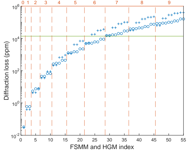
FIG. 7. Diffraction losses obtained for FSMM (cross) and estimated for HGM (circles). The vertical red dashed lines underline the mode orders, which appear in the upper horizontal axis. The horizontal lower axis shows the optical mode index (modes are sorted by increasing energies). The green line shows the input mirror transmittance.
