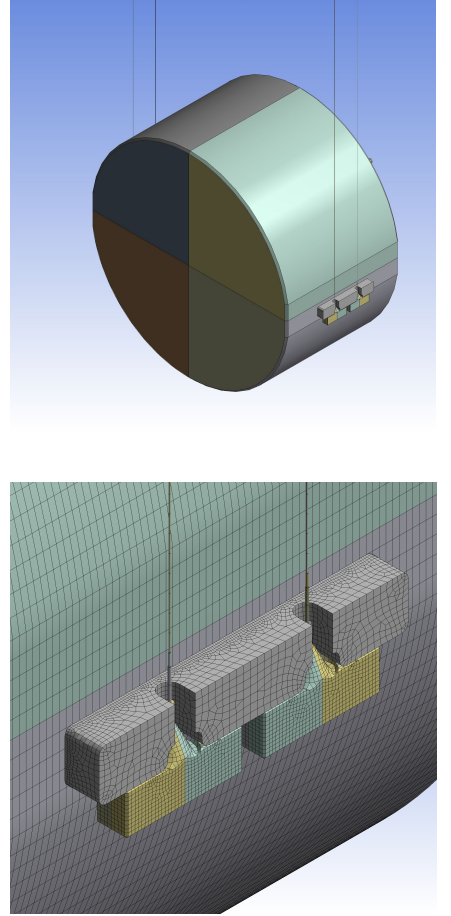
FIG. 2. Geometry used for the FEA, including the ears, the anchors and the magnets attached on the mirror rear face. The suspension wires are just for sketching but not included in the simulation as they do not influence the modal frequencies
