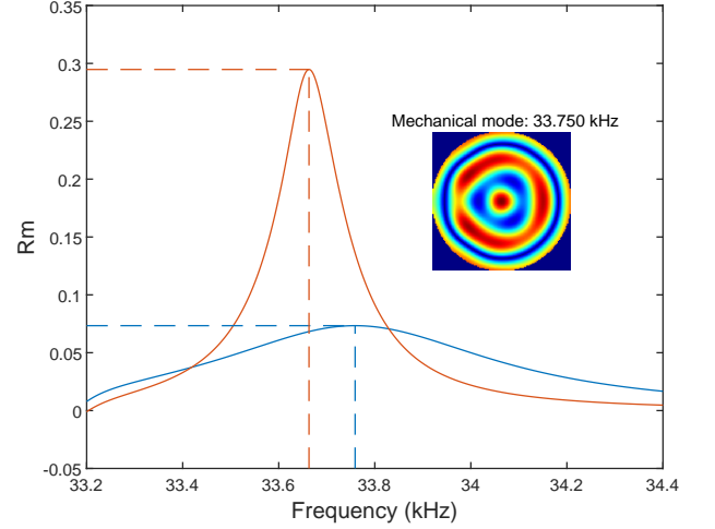
FIG. 12. Parametric gain R_m of the 33.750 kHz mechanical mode (see inset) while artificially varying the mechanical frequency, using the two different optical mode basis (red: HGM, blue: FSMM). The dashed lines point the maxima of the two curves, and emphasize the height and frequency change.
