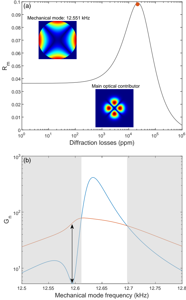
FIG. 11. (a) Parametric gain R_m of a mechanical mode of frequency 12.551 kHz while varying artificially the diffraction losses of optical modes. (b) Optical gain G_n of a FSMM high order mode versus the mechanical mode frequency, which is artificially varied around the resonance condition \delta\omega = \omega_m (with \delta\omega = 12.551 kHz). The blue line is for null diffraction losses, and the red one is for 21540 ppm (red bullet at the maximum of the curve in (a)). The arrow points the minimum in between the two resonance on the blue curve, where the gain increase is maximum. The gray shaded area highlights a frequency at which G_n is higher when the diffraction loss is higher.
