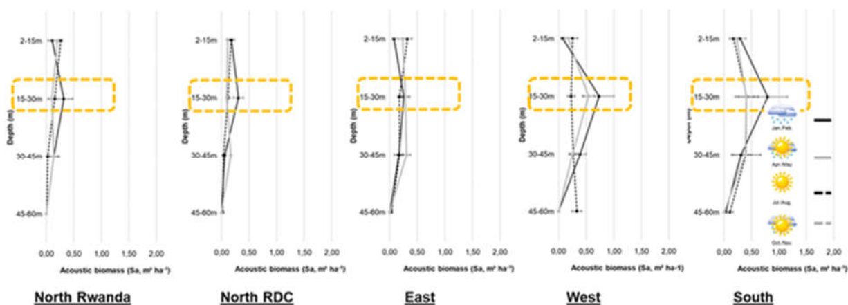
Figure 27 : fish distributions according to depth in the different basins of Lake Kivu in 2014
