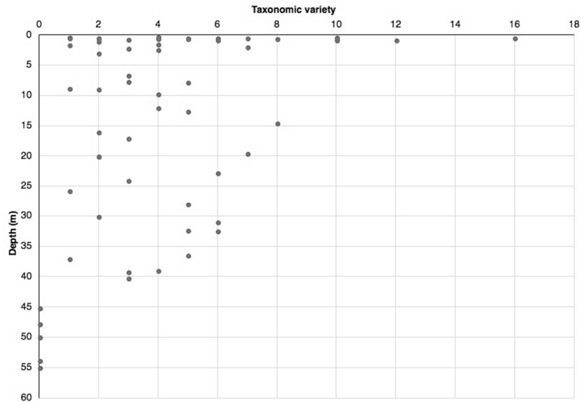
Figure 16 : Taxonomic diversity according to depth (63 samples).
