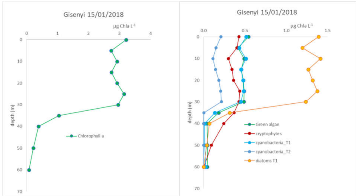
Figure 3: Vertical profiles of phytoplankton abundance in Lake Kivu, January 2018. Right: profiles of the main groups (green algae, cryptophytes, cyanobacteria type 1 & 2, diatoms type 1); Left: profile of chlorophyll a. The chlorophyll a profile suggests that the mixed layer was approximately 30 m. These results were obtained during the second mission in 2018, by Eric Mudakikwa, with the help of J.-P. Descy and Bruno Leporcq.
