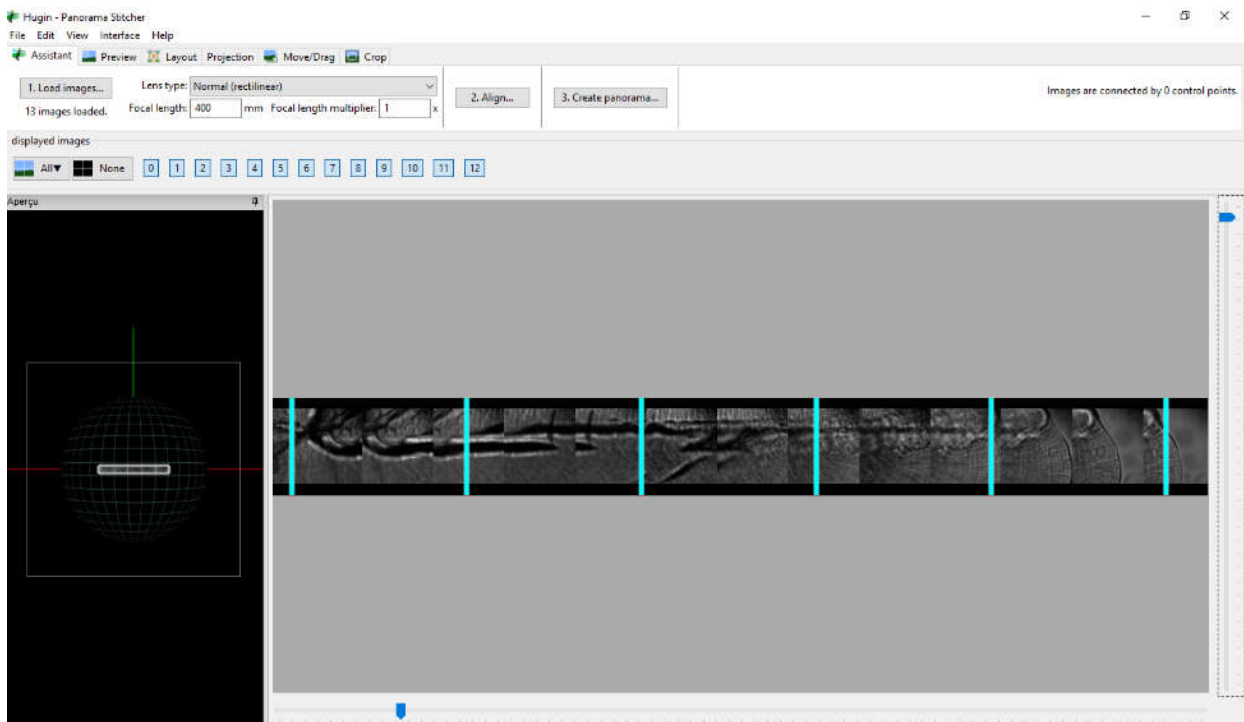
Figure 43 : Otolith pictures after upload in Hugin software (Picture M. Hautier)
