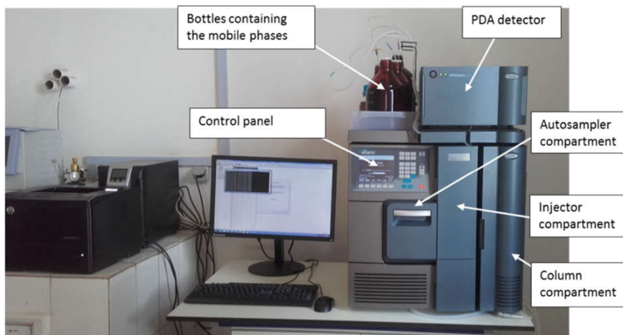
Figure 1: Picture of the Waters Alliance HPLC system installed in the LKMP lab at Cape Rubona.
