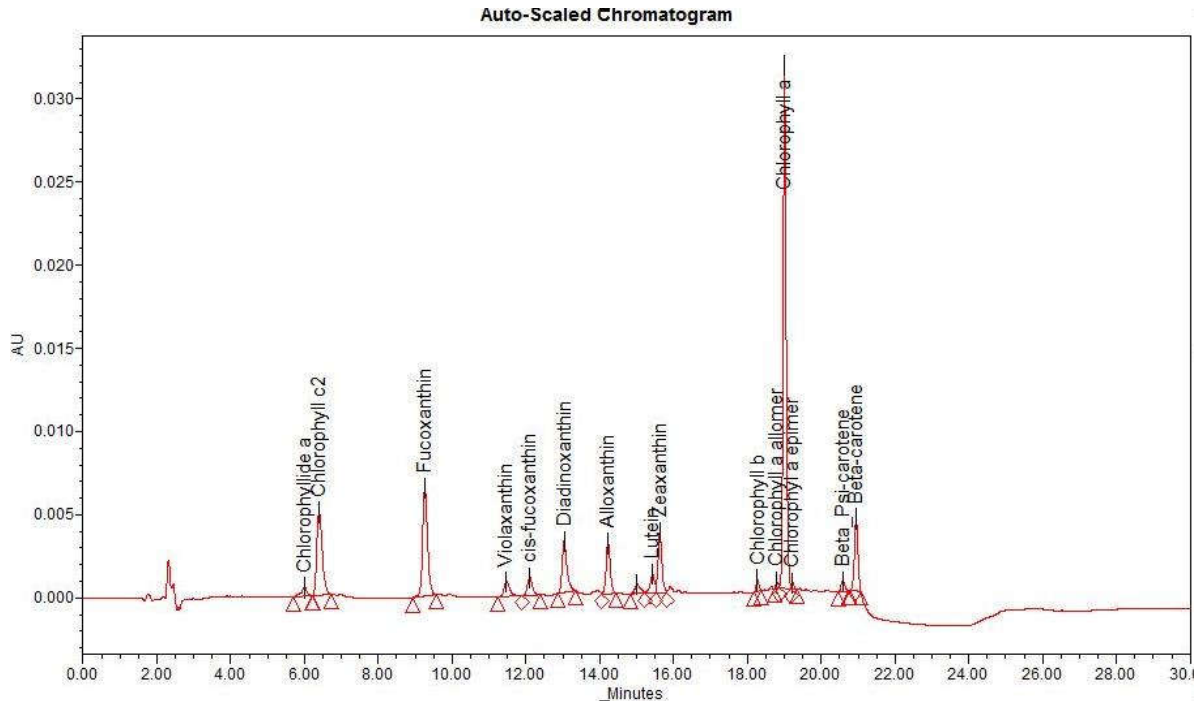
Figure 2: Example of a typical chromatogram obtained with the LKMP Alliance HPLC system, after processing for pigment identification. The major peak, with a retention time of ~19 min, corresponds to chlorophyll a, which is present in all phytoplankton groups. In this example, the sample contained mainly diatoms (with fucoxanthin and diadinoxanthin as markers), cryptophytes (alloxanthin), green algae (lutein and chlorophyll b), and cyanobacteria (zeaxanthin).
