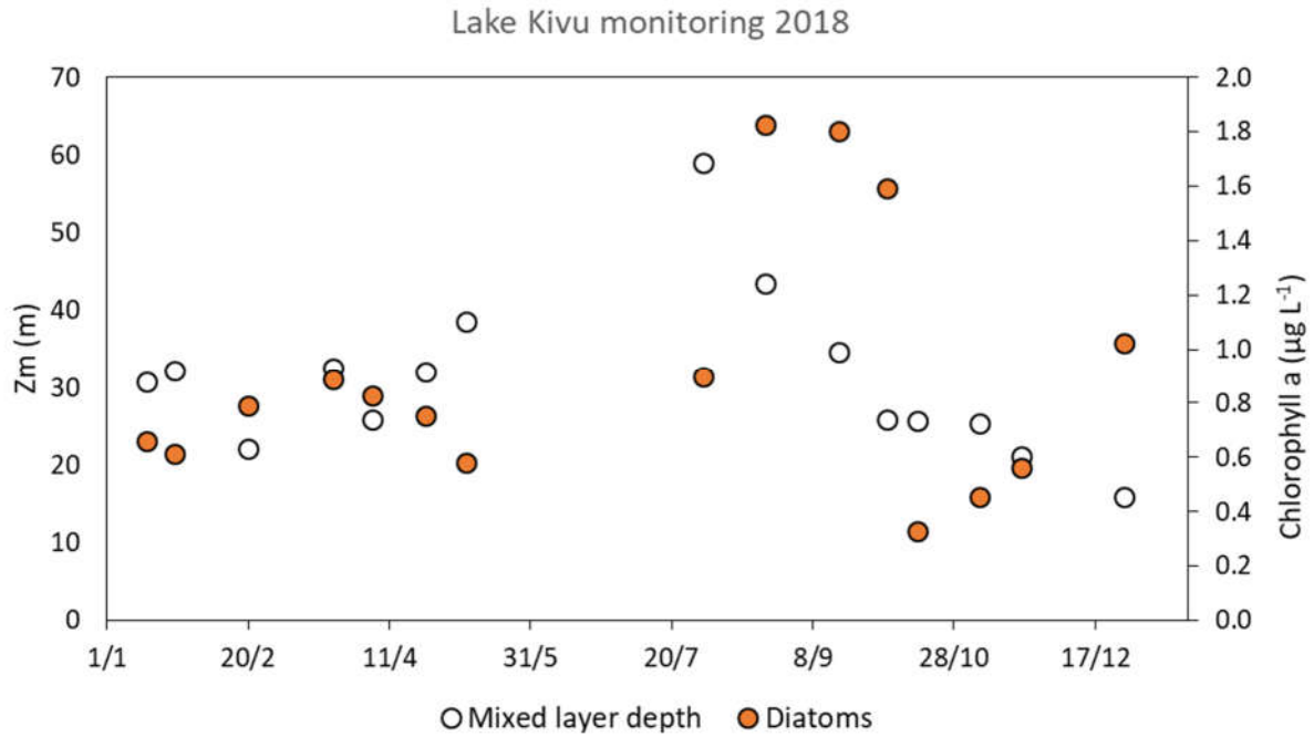
Figure 6 : Plot of diatom biomass (brown dots), expressed in chlorophyll a units ( \mu\text{g L}^{-1} ), vs. the Z_m (depth of the mixed layer) in Lake Kivu, 2018, off Gisenyi and Kibuye.
