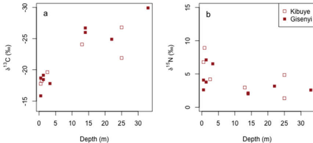
Figure 64. Relations between a) \delta^{13}\text{C} and b) \delta^{15}\text{N} and sampling depths for benthic macroinvertebrates
