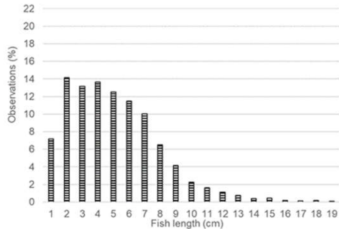
Figure 28 : Example of fish distributions in the North basin in July 2014 showing a bimodal distribution and a high proportion of small fish.
