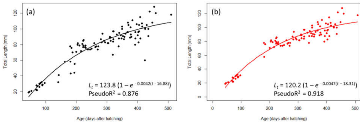
Figure 47 : Growth curve of L. midon using standard Von Bertalanffy model, considering: (a) all the dataset; (b) after removal of slow-growing individuals captured close to the shore
