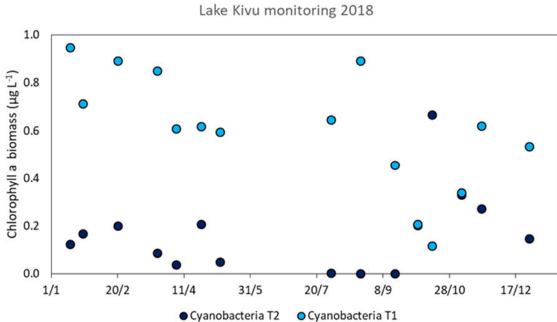
Figure 8 : Plot of cyanobacteria biomass, expressed in chlorophyll a units ( \mu\text{g L}^{-1} ) in Lake Kivu, 2018, off Gisenyi and Kibuye.
