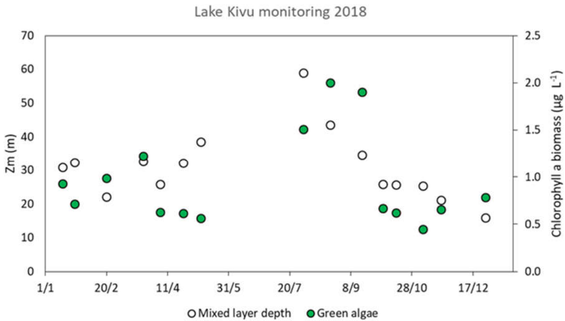
Figure 7 : Plot of green algae biomass (green dots), expressed in chlorophyll a units ( \mu\text{g L}^{-1} ), vs. depth of the mixed layer in Lake Kivu, 2018, off Gisenyi and Kibuye.
