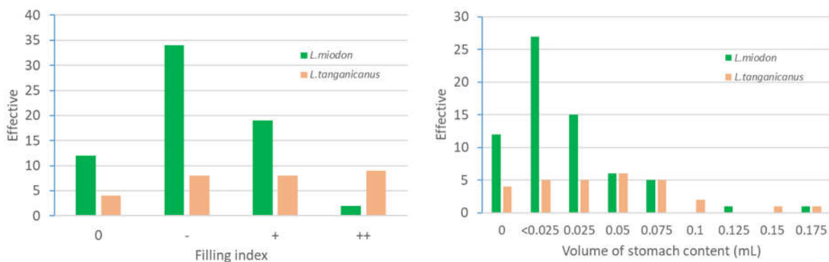
Figure 60 : (left) stomachs filling (“0” for empty; “-“ for almost empty, “+“ means that the stomach contains few preys, ++ means that the stomach contains several preys; (right) volumes distribution of the whole gut contents
