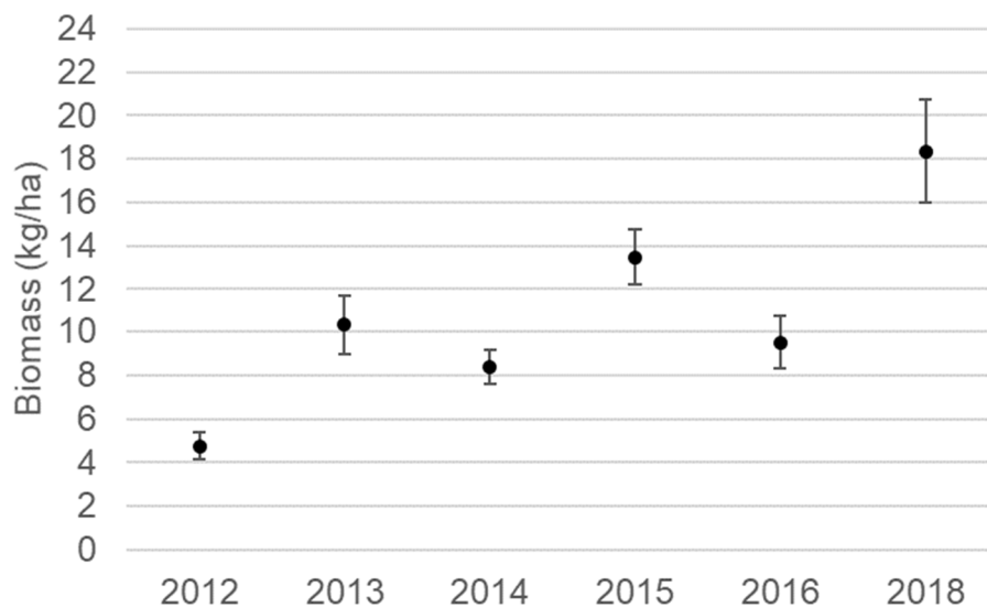
Figure 31 : Biomass ( kg \cdot ha^{-1} ) of Lake Kivu by year with confidence interval at 95%
