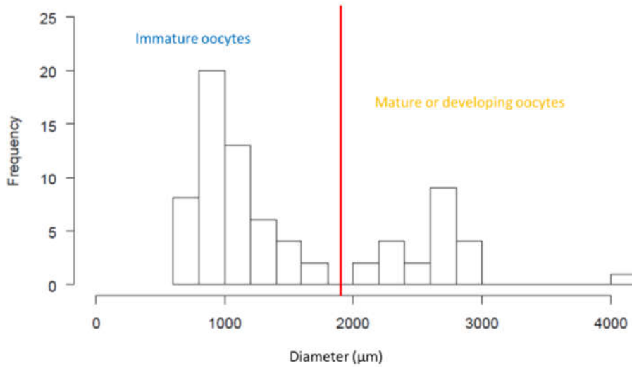
Figure 55 : Egg size distribution of a mature female L. tanganicus (TL = 85 mm)
