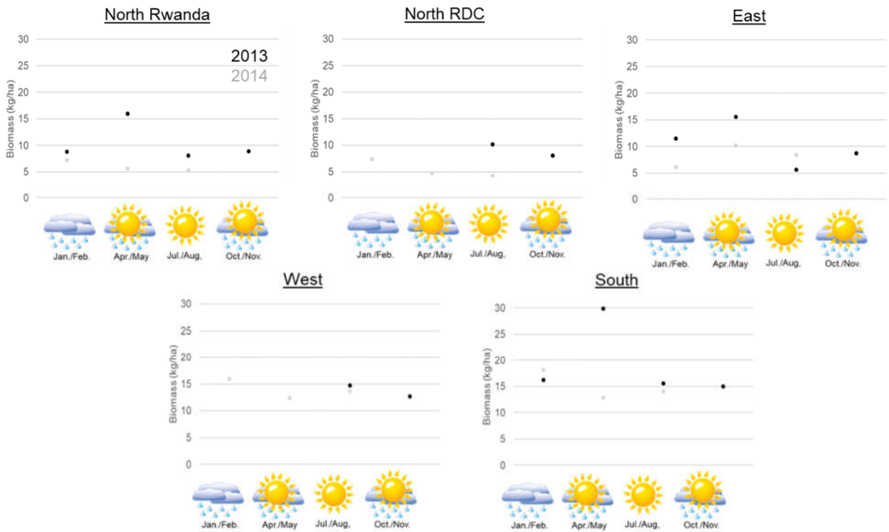
Figure 29 : Fish biomass by basin and by season in 2013 and 2014.
