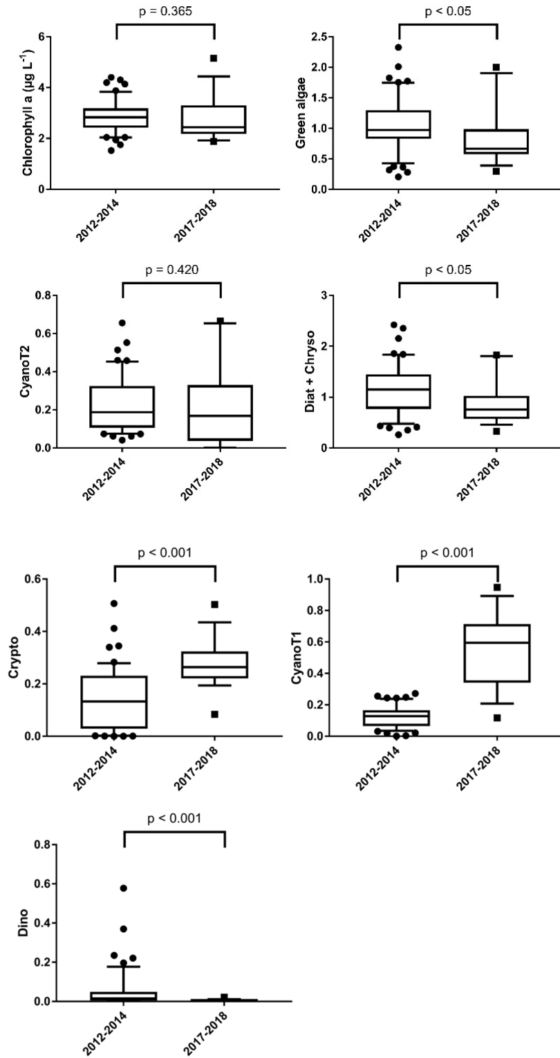
Figure 10 : Box-plots of chlorophyll a ( \mu\text{g L}^{-1} ) and biomass phytoplankton groups ( \mu\text{g chlorophyll a L}^{-1} ) in Lake Kivu, from the lake's monitoring off Kibuye and Gisenyi in 2012-2014 and in 2017-2018. Crypto = Cryptophytes; CyanoT1 = cyanobacteria T1; CyanoT2 = cyanobacteria T2; Diat+Chryso = diatoms + Chrysophytes; Dino = dinoflagellates. A Mann-Whitney test was applied to assess the significance of the difference between the two periods.
