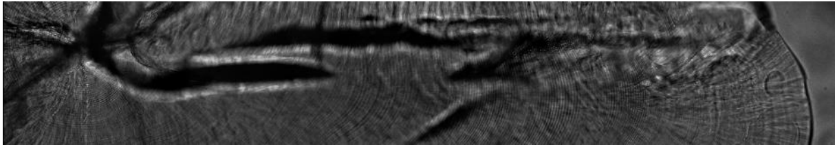
Figure 44 : Picture assembling of a sagittae of L. miodon along the main axis (Picture M. Hautier)
