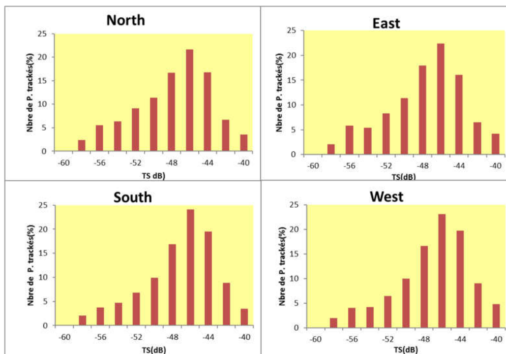
Figure 26: Fish size distributions in the four basins of Lake Kivu
