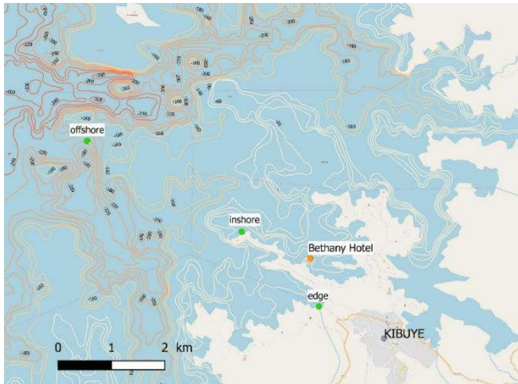
Figure 33: Location of the sampling sites (green dots) in Kibuye in July 2018
