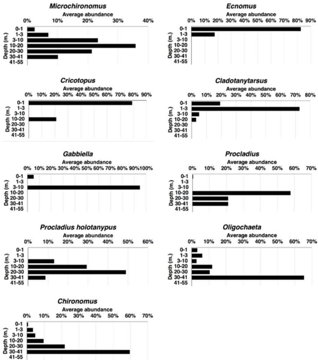
Figure 21 : Distribution according to depth of the most occurrent taxa
