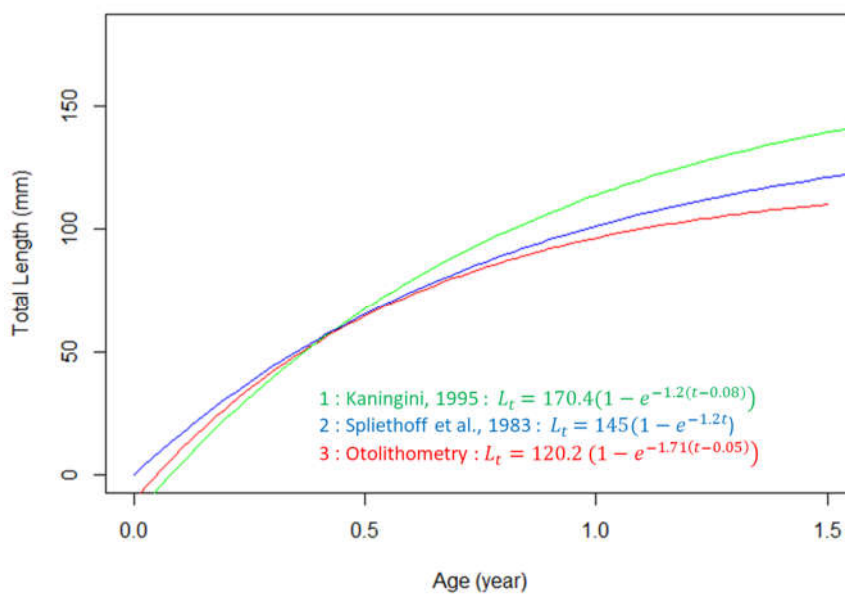
Figure 50 : Von Bertalanffy growth models of L. miodon in Lake Kivu
