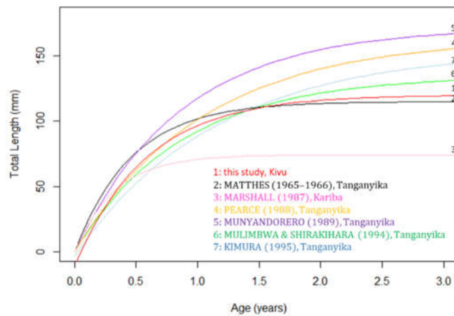
Figure 51 : Von Bertalanffy growth models of L. miodon in other African lakes
