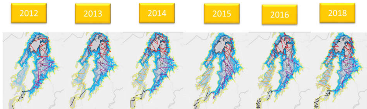
Figure 30 : Tracks performed during July-August hydroacoustic surveys from 2012 to 2018
