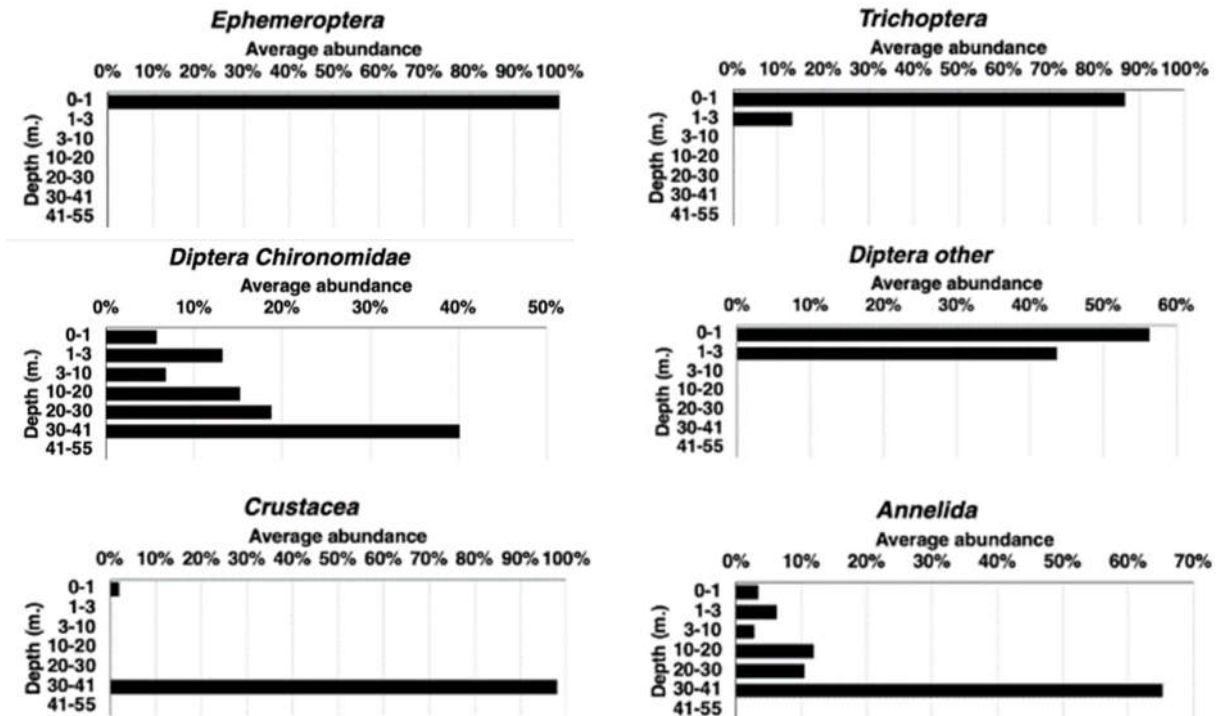
Figure 20 : Distribution according to the depth of 6 groups
