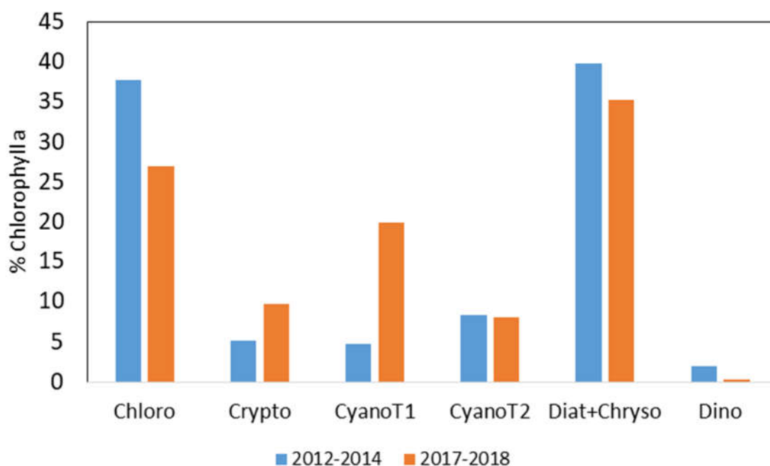
Figure 9: Mean contribution to chlorophyll a of the main phytoplankton groups, as estimated from the marker pigment concentrations processed with CHEMTAX: Comparison between the monitoring of Lake Kivu in 2012-2014 and in 2017-2018. Chloro = green algae; Crypto = Cryptophytes; CyanoT1 = cyanobacteria T1; CyanoT2 = cyanobacteria T2; Diat+Chryso = diatoms + Chrysophytes; Dino = dinoflagellates.
