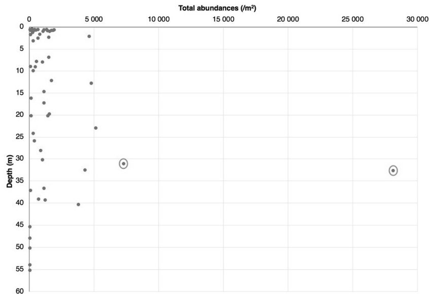
Figure 17 : Numerical abundance of macroinvertebrates (ind / m 2 ) in samples according to depth (63 samples).
