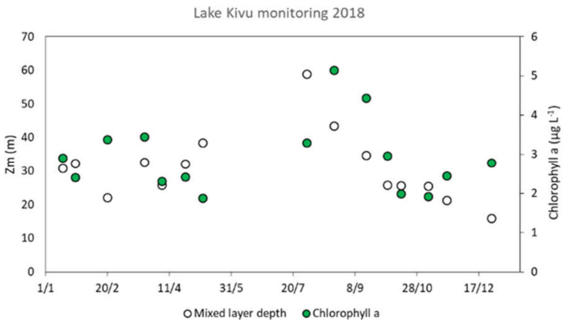
Figure 5 : Plot of chlorophyll a (i.e. total phytoplankton biomass) vs. depth of the mixed layer in Lake Kivu, 2018, off Gisenyi and Kibuye.
