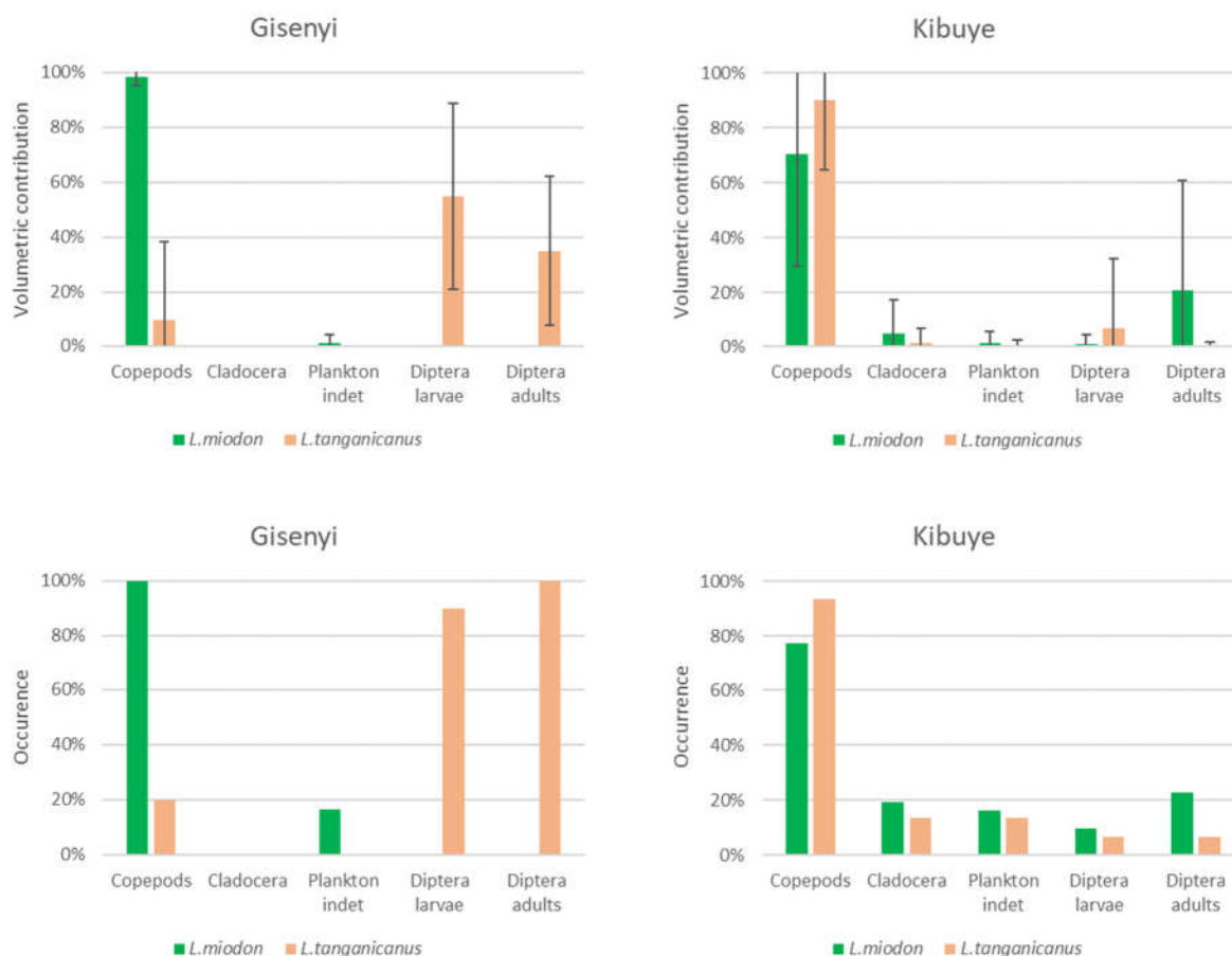
Figure 61 : Mean \pm SD volumetric percentages (up) and occurrence (down) of the main prey taxa found in the stomachs of the 2 fish species, collected in the inshore areas of the 2 sites.
