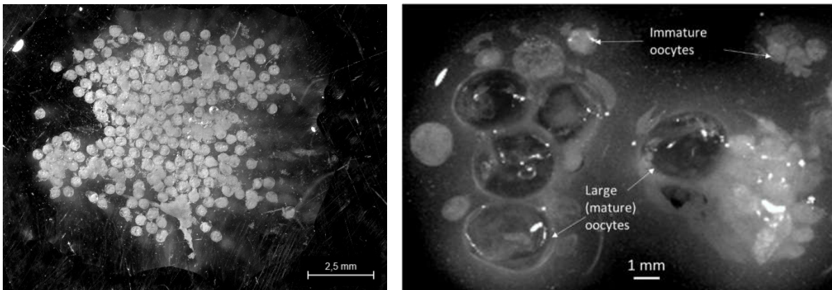
Figure 54 : homogeneous oocytes sizes for L. miodon (left) and different stages of oocytes development in L. tanganicanus (right). Pictures A. Reveret.
