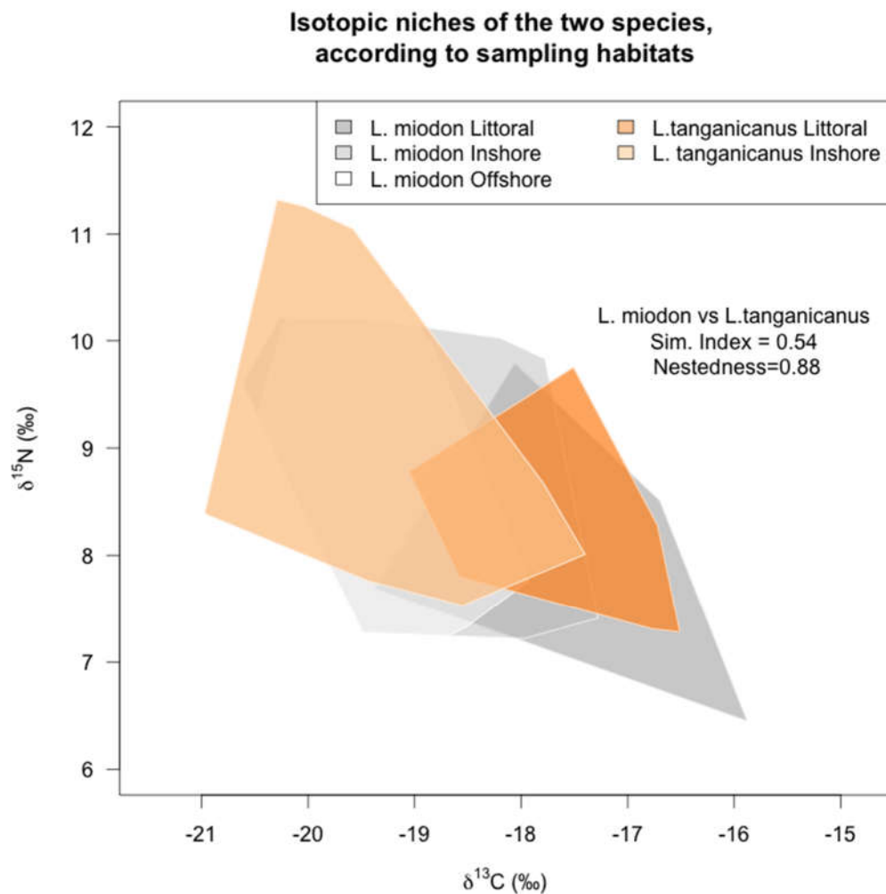
Figure 68. Comparison of the isotopic niche of both species. *ISim (isotopic similarity) = ratio between the volume of the intersection and the volume of the union of the two groups of organisms in the stable isotope space. ** INes (isotopic nestedness): ratio between the volume of the intersection and the minimal volume filled by a group (Cucherousset & Villéger, 2015)
