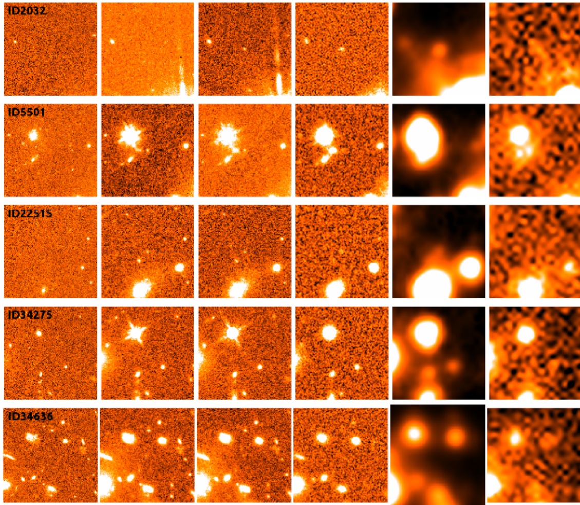
Figure E1. Snapshots of the five passive candidates selected with the \tau -models library which are not present in the reference sample. Left to right: ACS B435 + V606 + I814 stack, WFC3 J125 , WFC3 H160 , Hawk-I Ks , IRAC 3.6 + 4.5 \mu\text{m} stack, IRAC 5.8 + 8.0 \mu\text{m} stack. [A colour version of this figure is available in the online version.]
