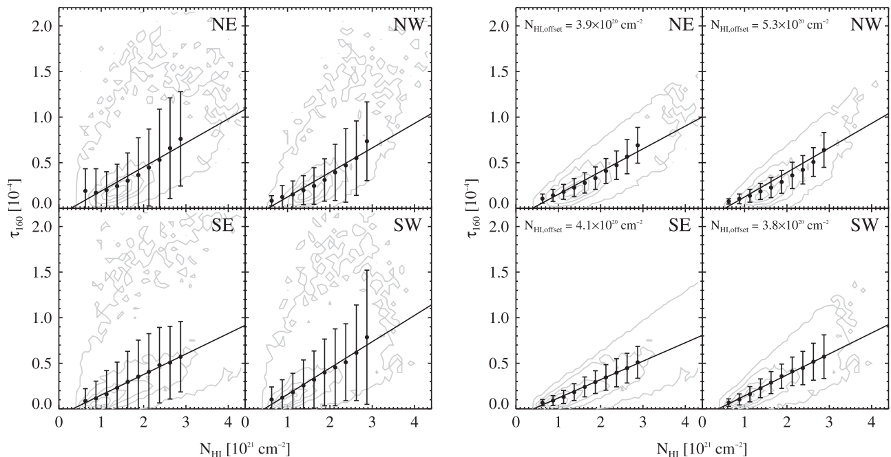
Figure 14. Same as Figure 13 but with \tau_{160} from the Gordon et al. (2014) dust modeling results.
