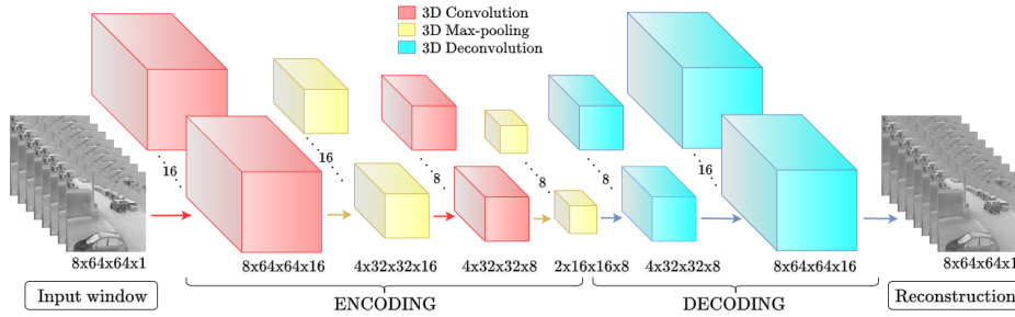
Fig. 1: Network architecture of DSTCAE-Deconvolution. The encoder is composed of layers with 3D convolution (red) followed by 3D max-pooling (yellow) and decoder is composed of 3D deconvolution (blue) layers. Each layer has dimensions: time window length \times height \times width \times number of feature maps.
