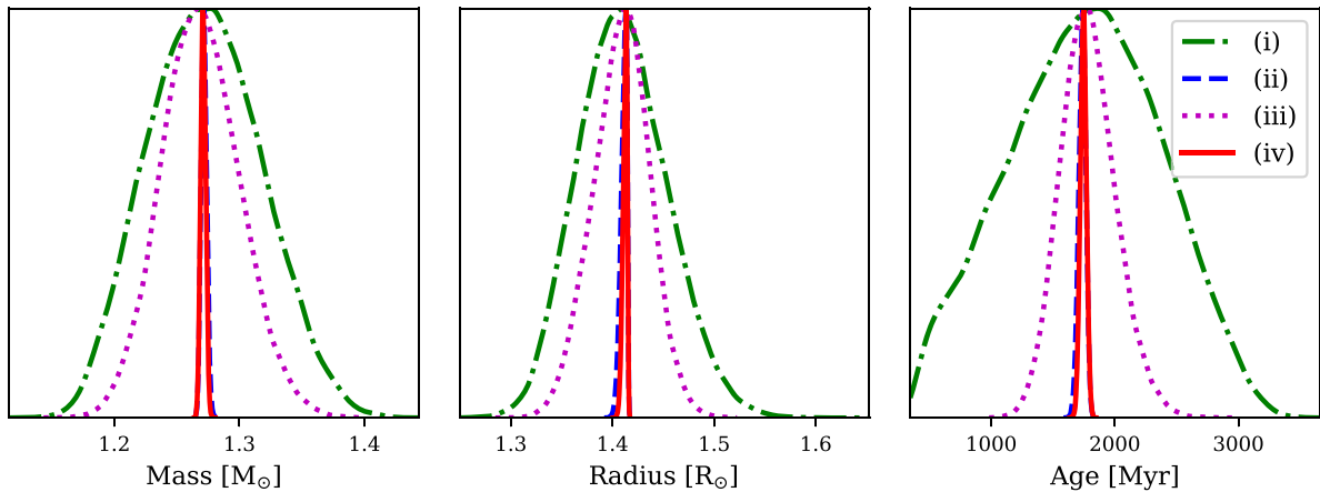
Figure 13. Comparison of input classical and seismic constraints for mass (left), radius (centre), and age (right) determination. The normalized distributions represent the different classical constraint criteria: (i) green, dot–dashed; (ii) blue, dashed; (iii) magenta, dotted; (iv) red, solid.
